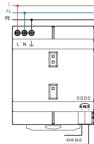
Wiring diagram for 78.2K
