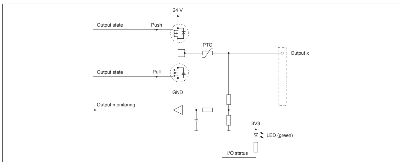
Figure 4: Input/Output circuit diagram of digital mixed channels (X1)
