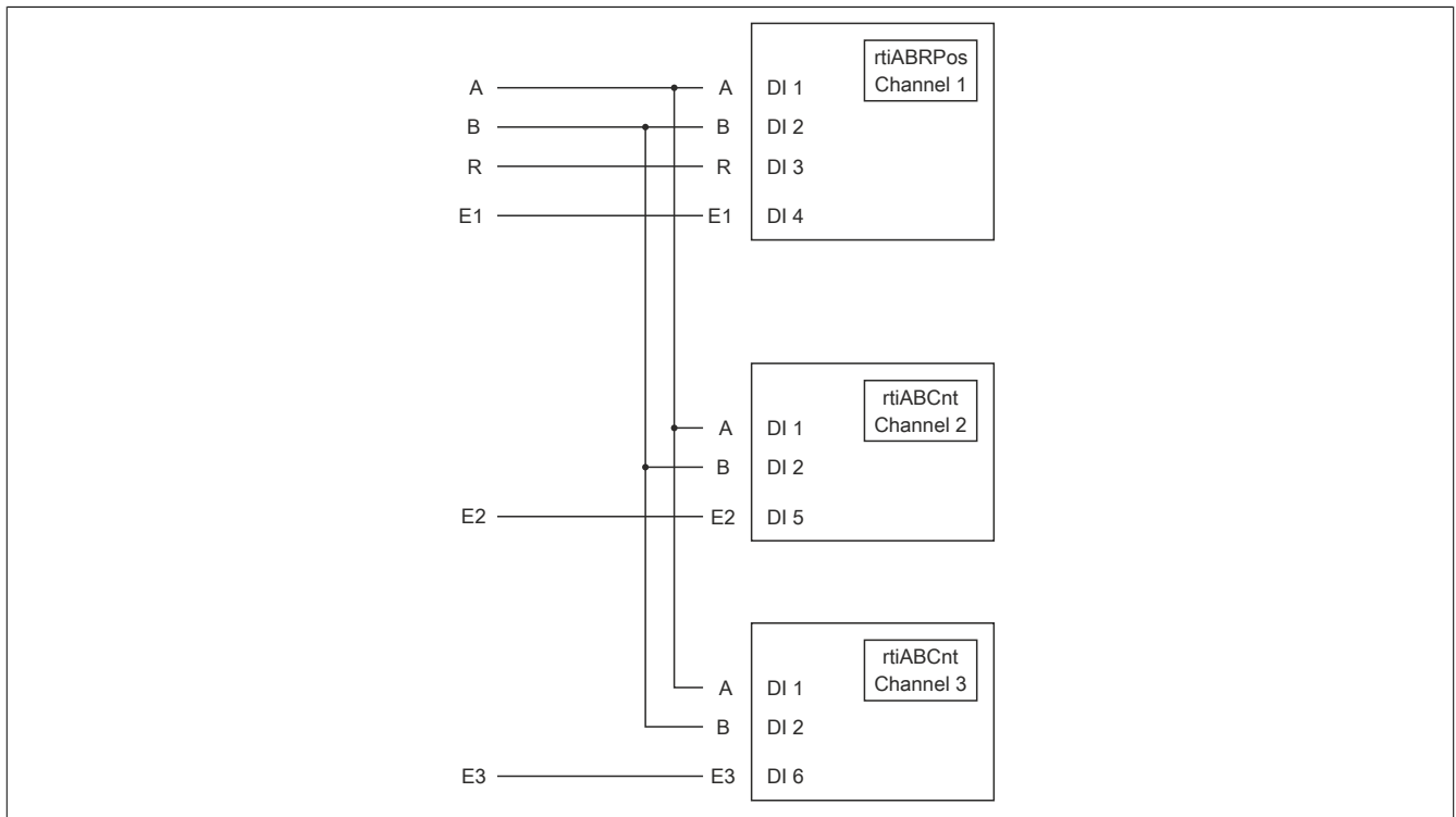
Figure 9: Diagram of input signals when using rtiABRPos and rtiABCnt at the same time
