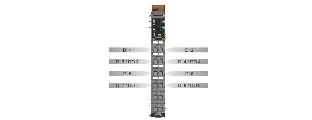
Figure 1: X1 - Pinout
