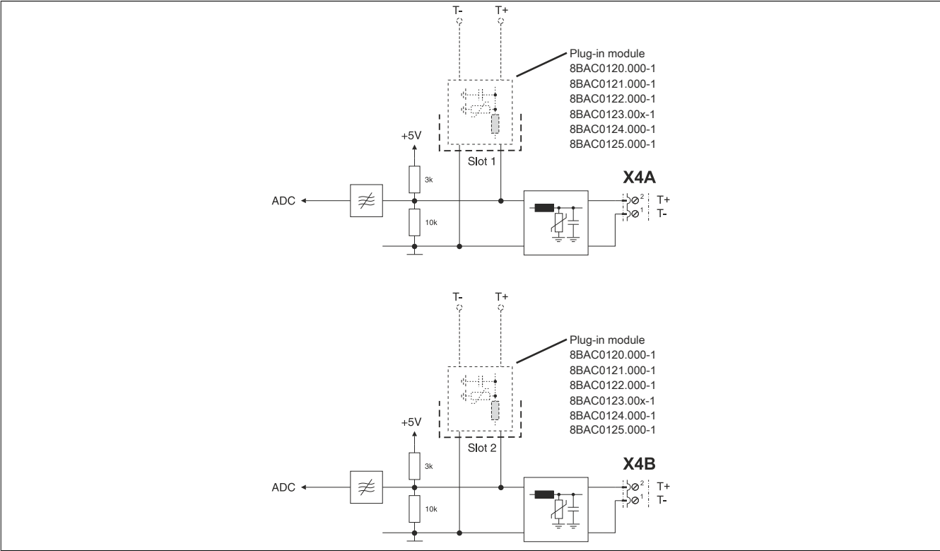
Figure 10: Temperature sensor
