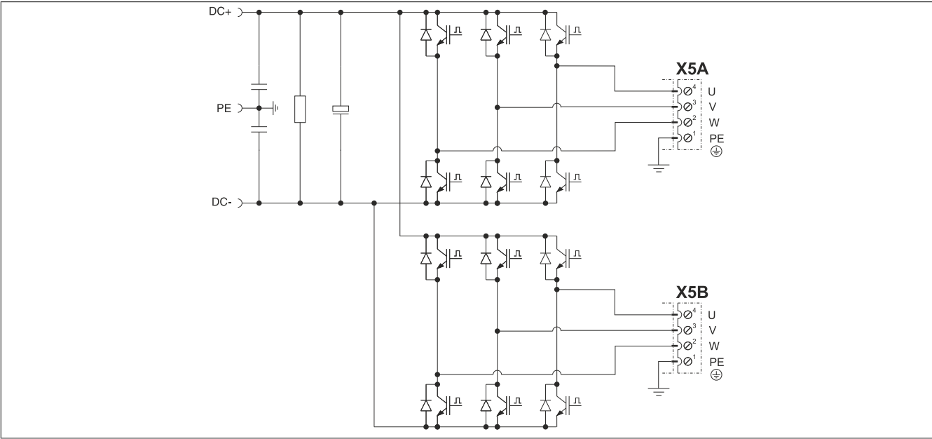
Figure 11: Motor
