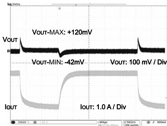
Fig.15 Transient Response (VIN= 12V Vout= 3.3V L= 10 \mu H Cout =22 \mu F Iout= 0.2-3.0A)
