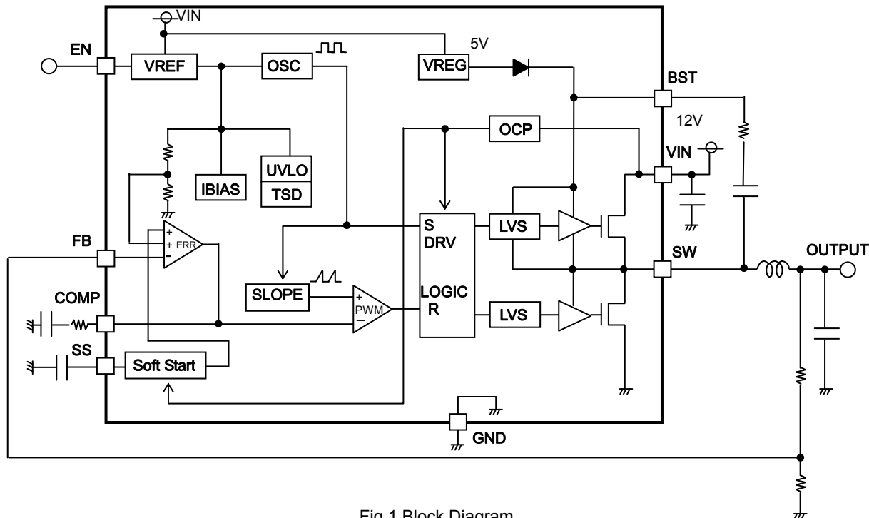
Fig.1 Block Diagram
