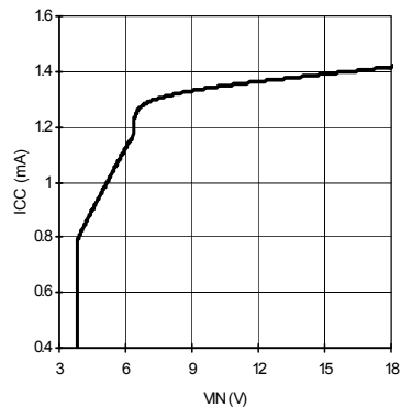
Fig.4 Circuit Current (No switching)
