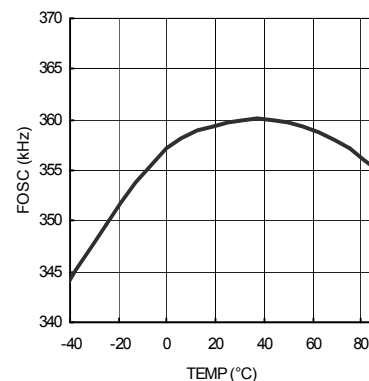
Fig.9 Operating Frequency
