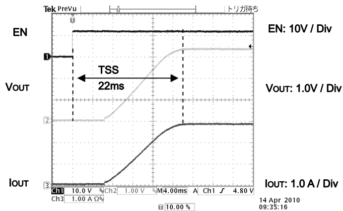
Fig.17 Start Up waveform (VIN= 12V Vout= 3.3V L= 10 \mu H C SS = 0.1 \mu F)
