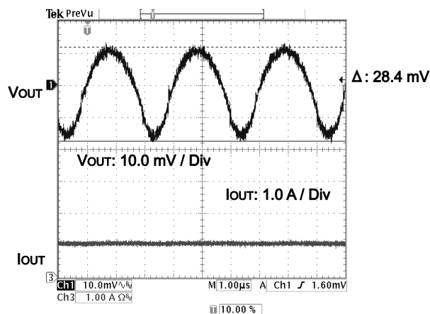
Fig.14 Output Ripple Voltage (VIN= 12V Vout= 3.3V L= 10 \mu H Cout =22 \mu F I out= 1.0A )
