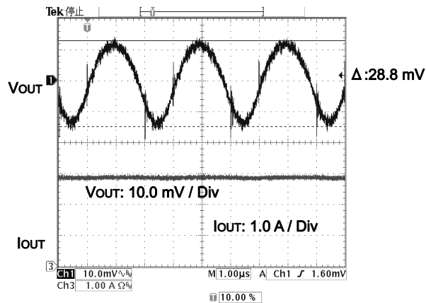
Fig.16 Output Ripple Voltage (VIN= 12V Vout= 3.3V L= 10 \mu H Cout =22 \mu F I out= 3.0A )
