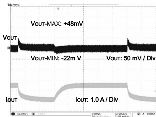
Fig.13 Transient Response (VIN= 12V Vout= 3.3V L= 10 \mu H Cout =22 \mu F Iout= 0.2-1.0A )
