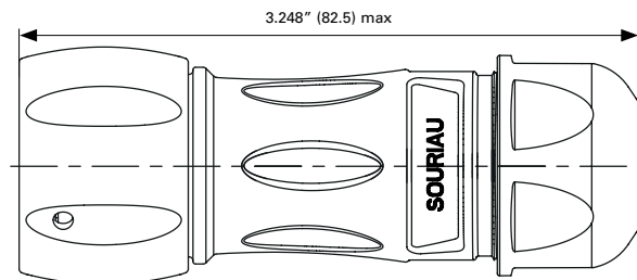
Fig.3 Cable diameter acceptance from 0.393" to 0.511" (10 to 13)
