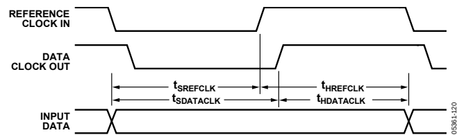
Figure 92. Timing Specifications, PLL Enabled or Disabled, Interpolation = 1x
