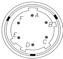
6 pin Connector VPT07RA10-6PT2 (PT02A-10-6P)
