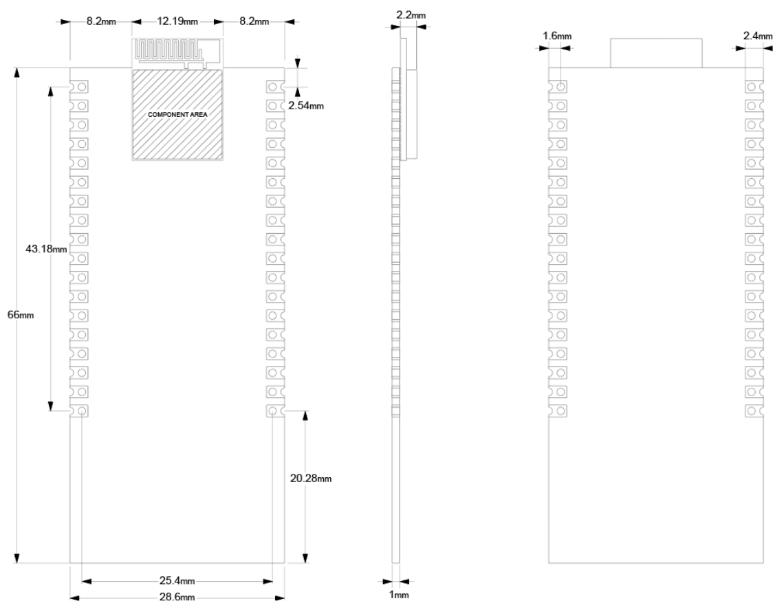
Figure 5: MQM711 Module Development Kit Dimension
