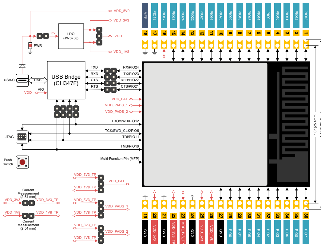
Figure 3: MQM711 Module Development Kit Block Diagram
