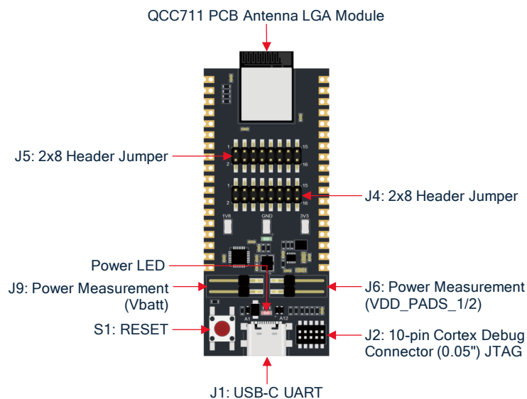
Figure 4: MQM711 Module Development Kit Component Layout
