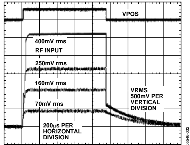
Figure 32. Output Response to Gating on Power Supply for Various RF Input Levels, Supply 3 V, Modulation Frequency 900 MHz, 0.01 \mu F Filter Capacitor
