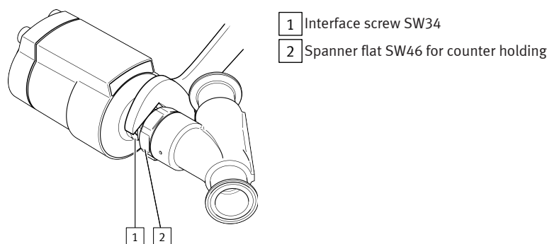
Fig. 2: Demounting drive
