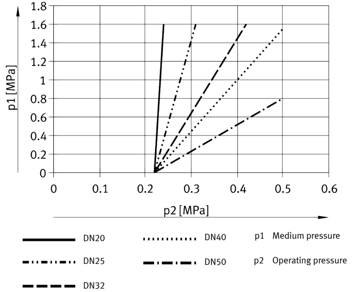
Fig. 5: Pressure of medium and operating pressure VZXA-A-...-K-75-...-PR
