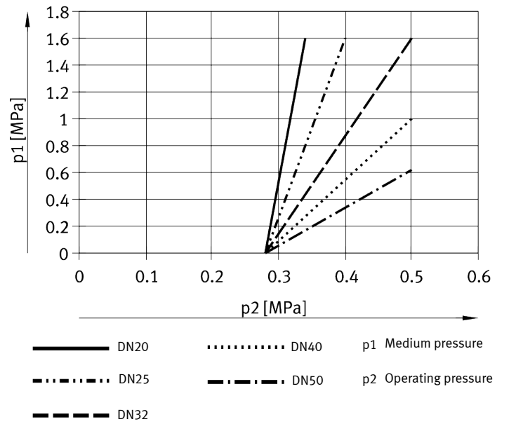
Fig. 3: Pressure of medium and operating pressure VZXA-B-...-K-75-...-S
