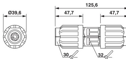
Dimensioned drawing
