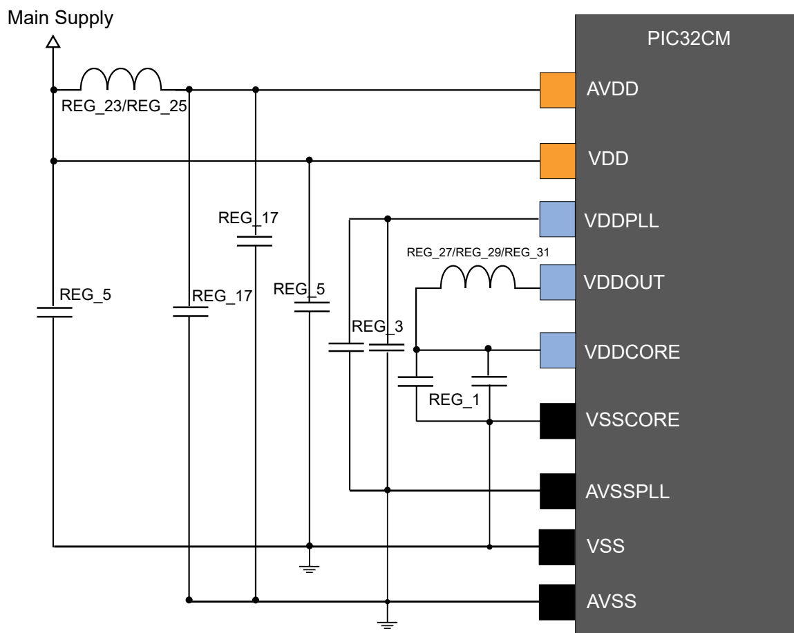
Figure 53-1. Power Supply Connection for Switching/Linear Mode
