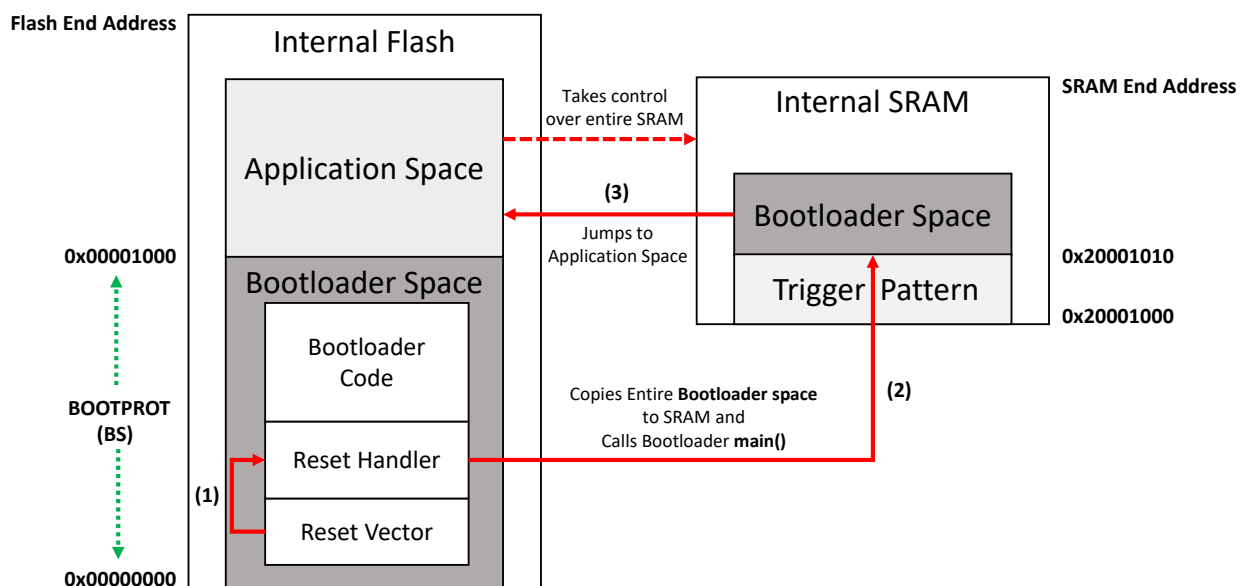
Figure 54-2. UART-I 2 C Bootloader Memory Layout For PIC32CM LS00/LS60
