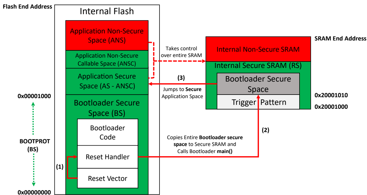
Figure 54-2. UART-I 2 C Bootloader Memory Layout For PIC32CM LS00/LS60
