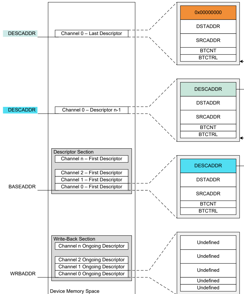
Figure 27-3. Memory Sections
