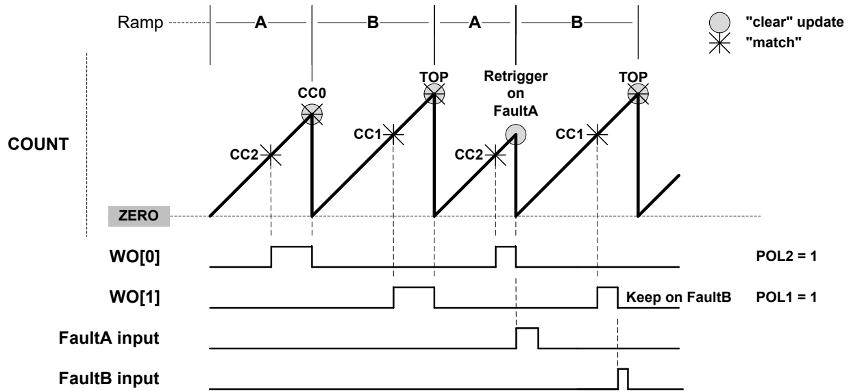
Figure 40-21. Critical RAMP2 Operation With More Than 2 Channels
