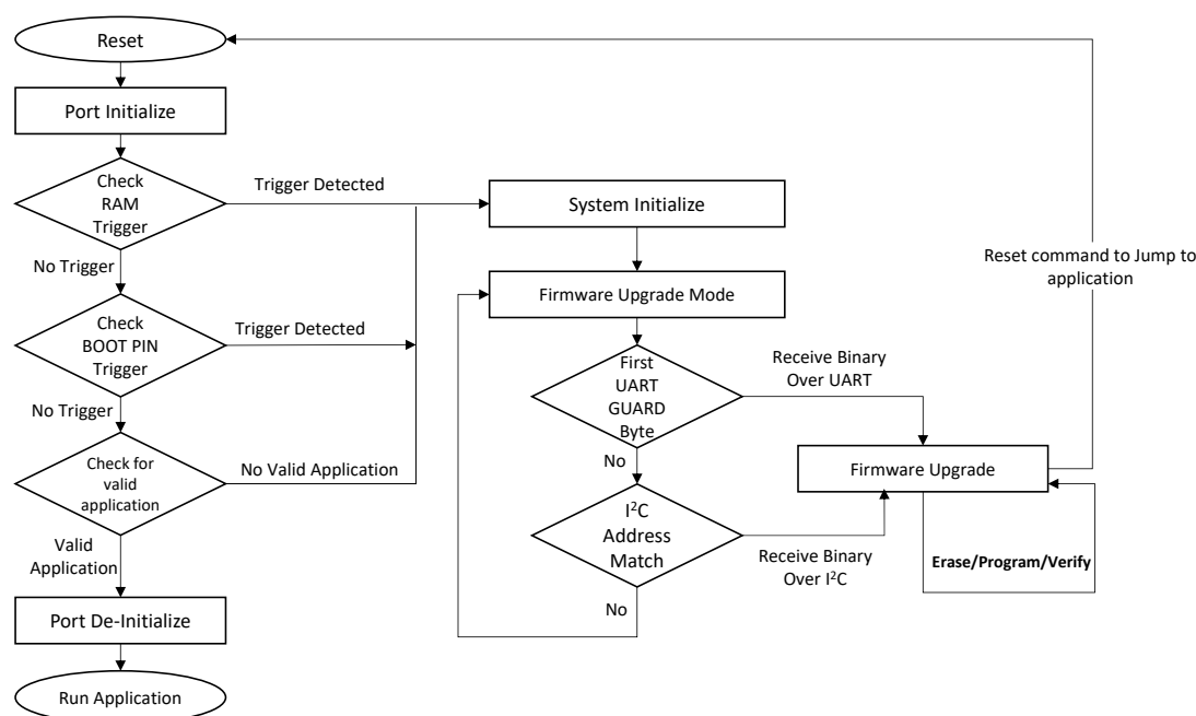
Figure 54-3. UART-I 2 C Bootloader System Level Execution Flow
