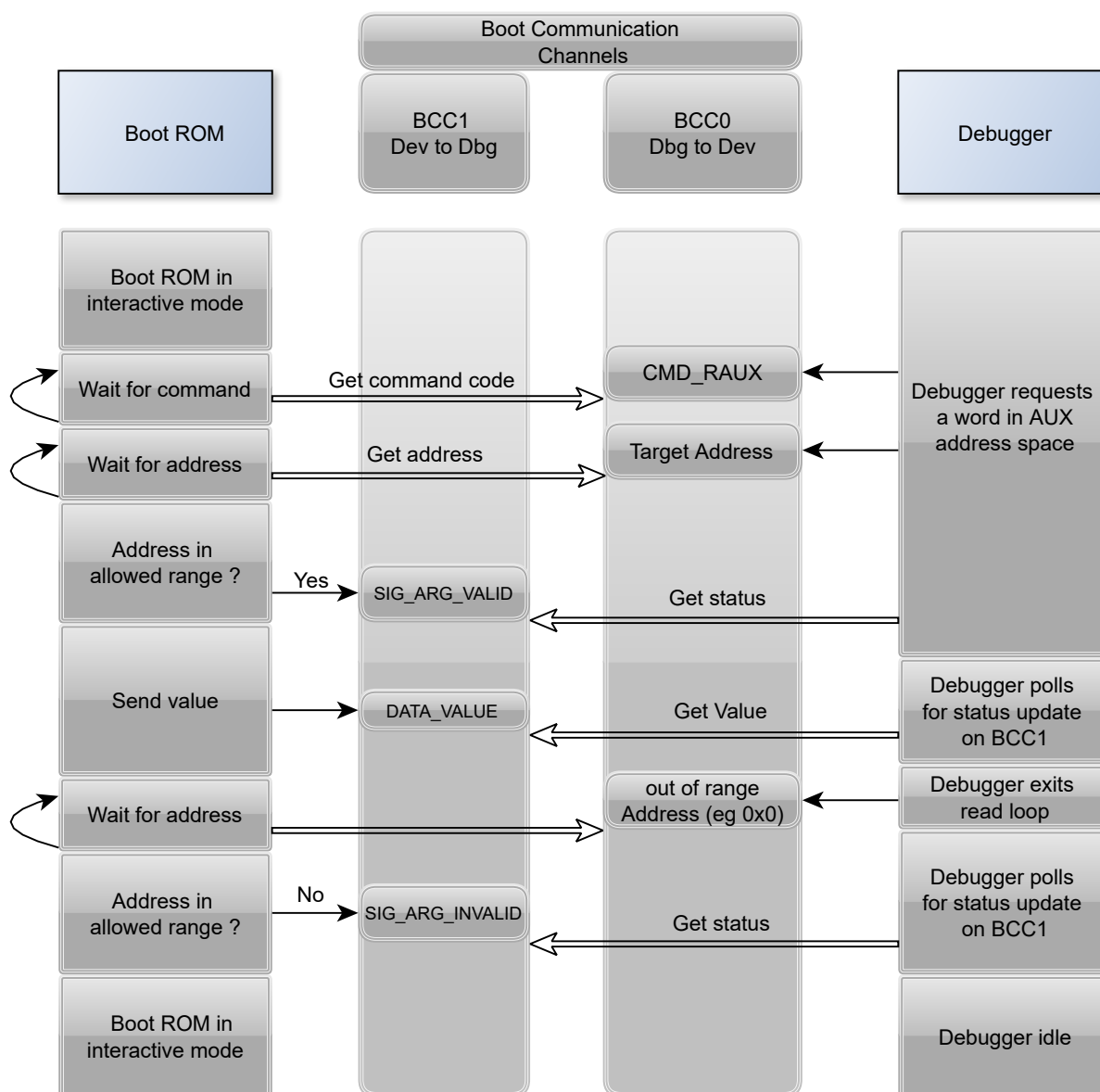
Figure 13-21. CMD_RAUX Flow diagram
