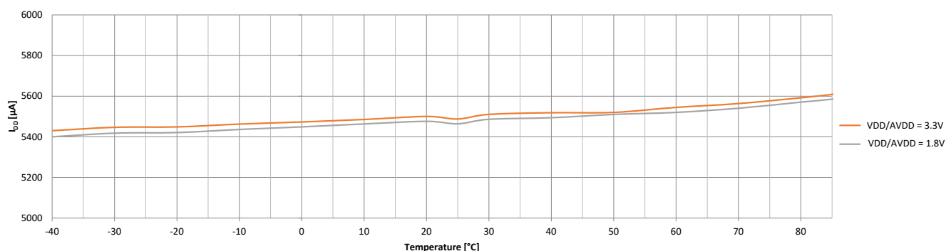
Figure 49-2. Power Consumption over Temperature in Active Mode (PL2 @48MHz)
