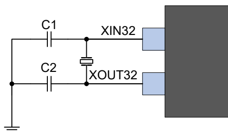
Figure 53-9. 32.768 kHz Crystal Oscillator Schematics
