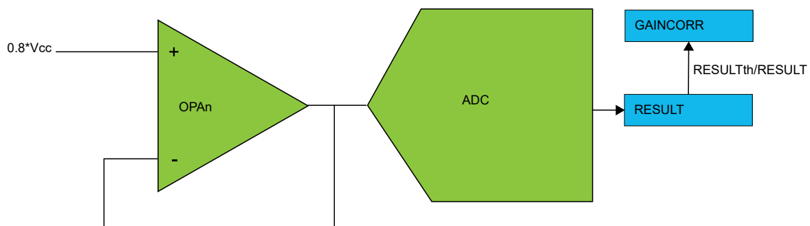
Figure 47-13. Gain Compensation
