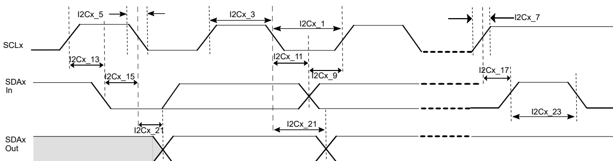
Figure 49-19. I 2 C Bus Data Client Mode Timing Diagrams
