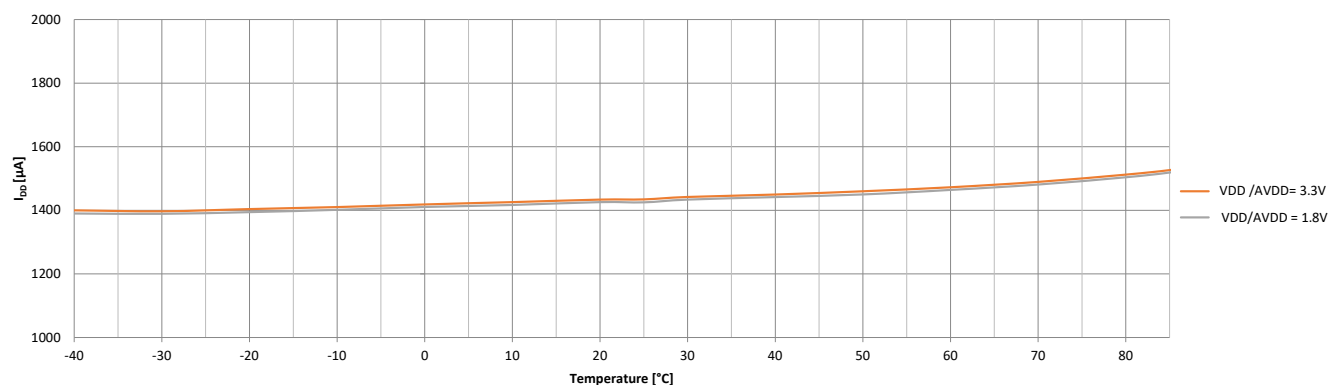
Figure 49-1. Typical Power Consumption over Temperature in Active Mode (PL0 @12MHz)
