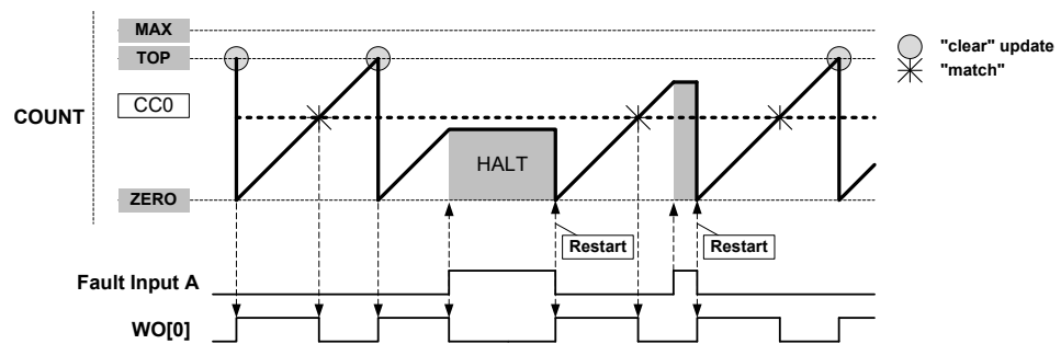
Figure 40-33. Waveform Generation with Fault Qualification, Halt, and Restart Actions
