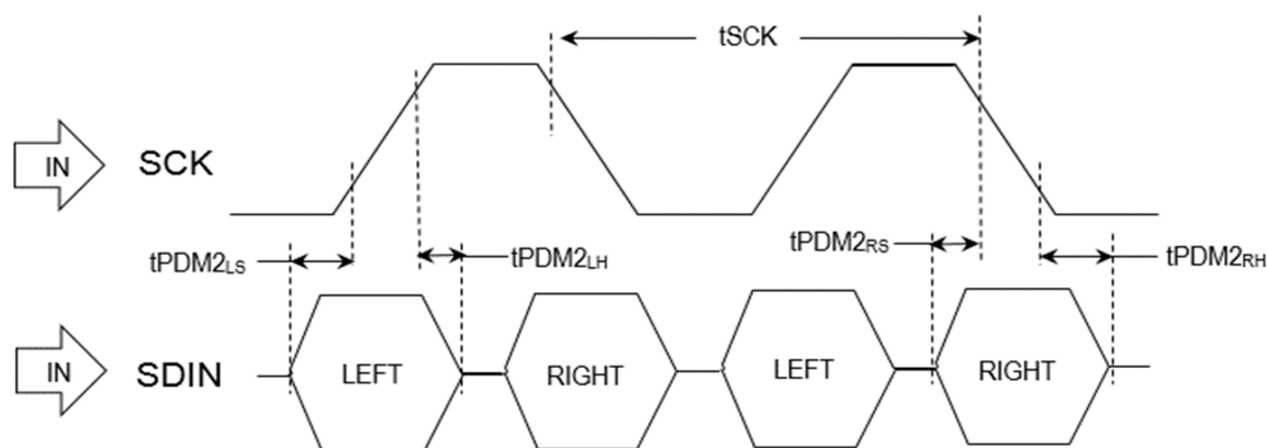
Figure 49-15. I 2 S PDM2 Mode Timing Diagram
