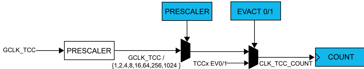
Figure 40-2. Prescaler
