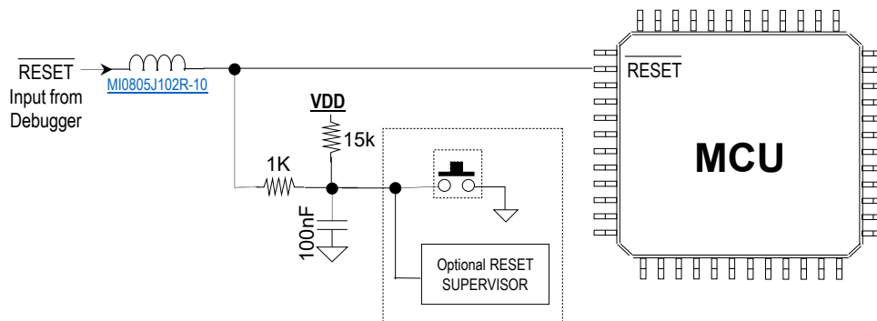
Figure 53-5. External Reset Circuit Schematic
