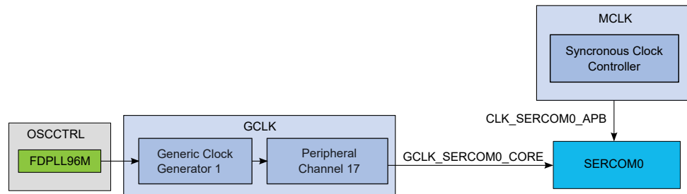
Figure 9-3. SERCOM0 Clock Distribution Example
