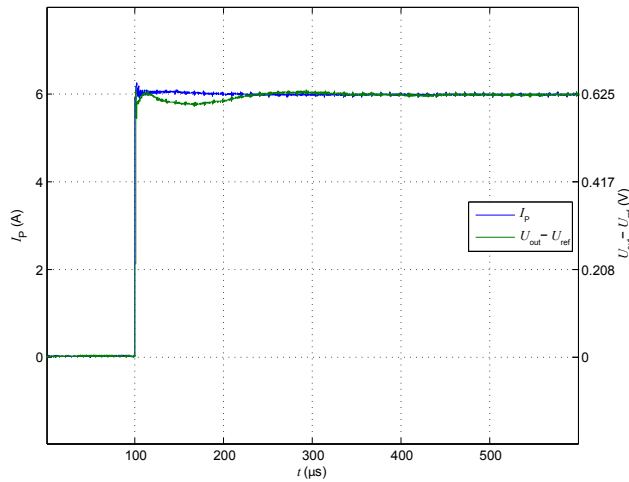
Figure 3: Step response
