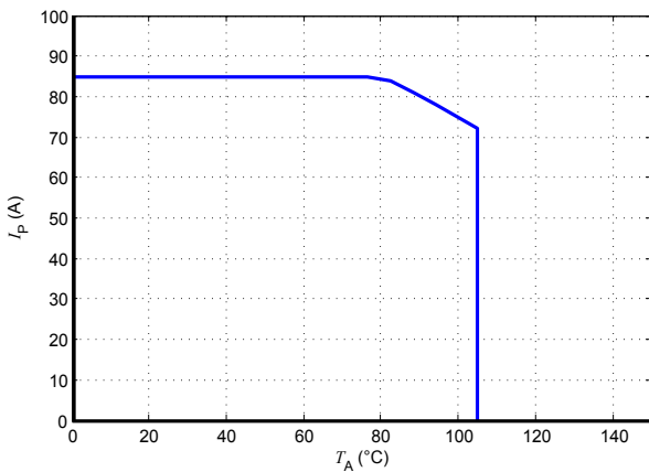
Figure 23: I p vs T A for LESR 25-NP
