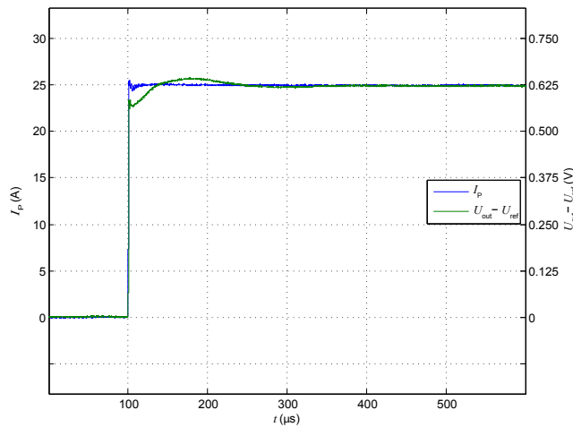
Figure 18: Step response
