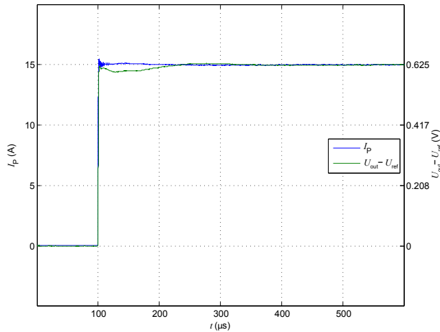
Figure 8: Step response
