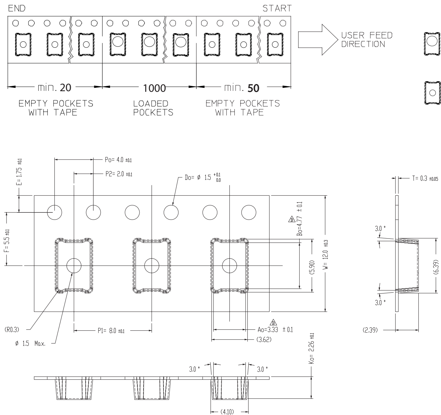
Figure 15. Emitter pocket tape packaging.
