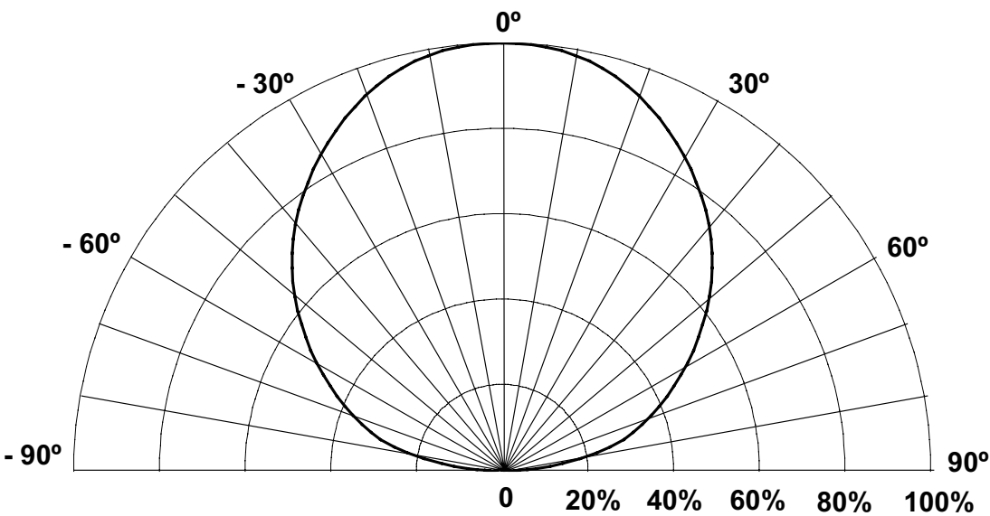
Figure 14. Typical polar radiation pattern for lambertian.
