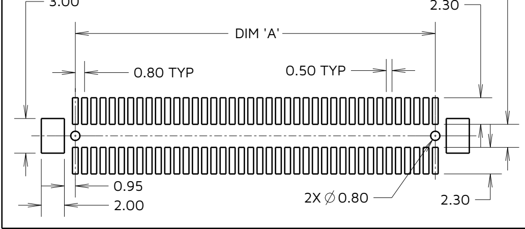
RECOMMENDED PCB LAYOUT (±0.05)
