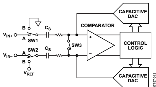
Figure 15. ADC Acquisition Phase
