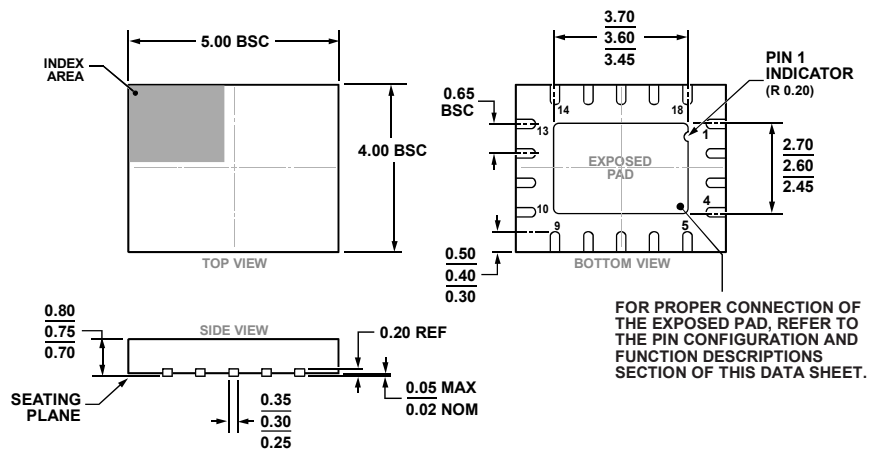
Figure 343. 18-Lead Lead Frame Chip Scale Package [LFCSP_WQ] 5mm x 4 mm Body, Very Very Thin Quad (CP-18-1)
