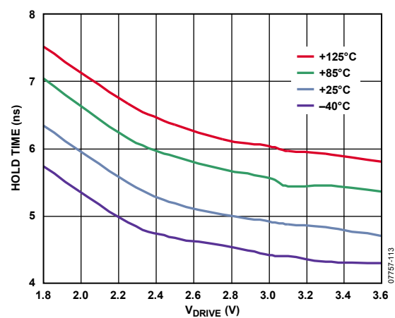
Figure 14. Hold Time vs. V_{DRIVE}
