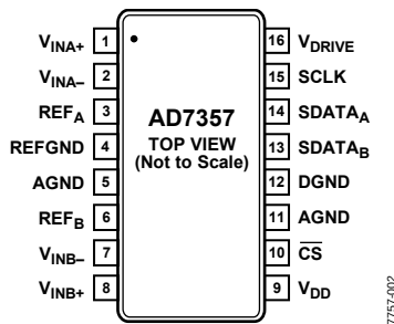
Figure 2. Pin Configuration, TSSOP
