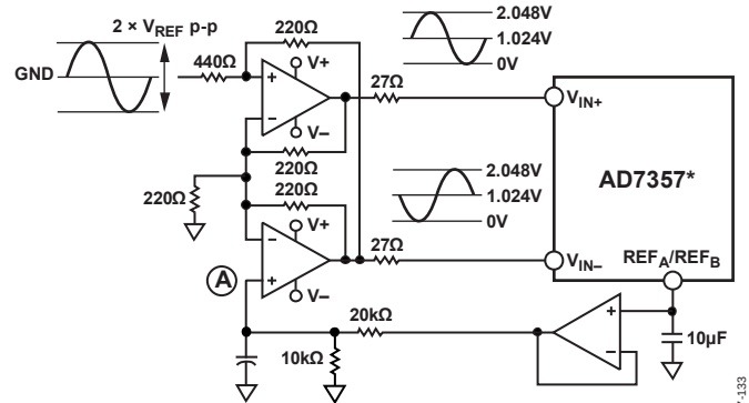
Figure 23. Dual Op Amp Circuit to Convert a Single-Ended Bipolar Signal into a Differential Unipolar Signal
