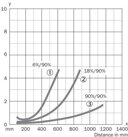
Figure 6: WT34-Xx4x, -Xx5x, red light
