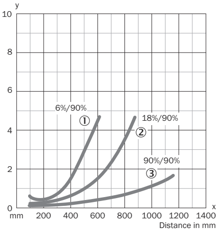
Figura 6: WT34-Xx4x, -Xx5x, luce rossa
