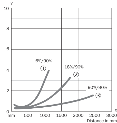
Illustration 7: WT34-Xx1x, -Xx2x, lumière infrarouge
