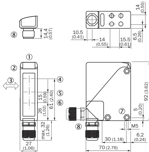
Illustration 9: Plan coté
