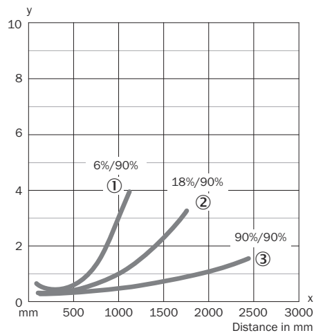
Figura 7: WT34-Xx1x, -Xx2x, luz infrarroja
