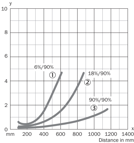
Illustration 6: WT34-Xx4x, -Xx5x, lumière rouge
