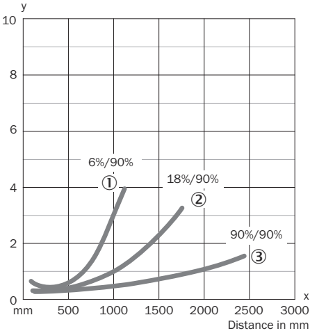
Figure 7: WT34-Xx1x, -Xx2x, infrared light
