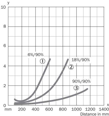
Figura 6: WT34-Xx4x, -Xx5x, luz roja
