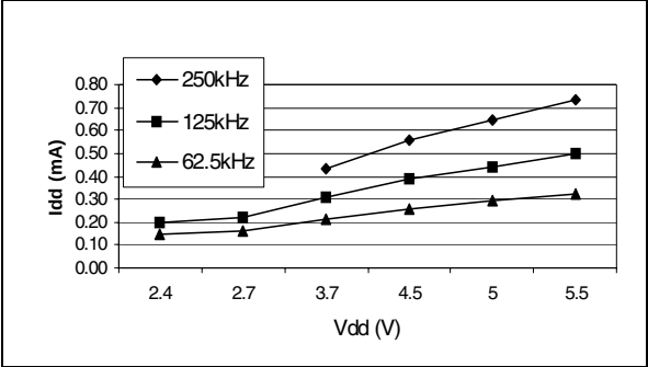
Figure 57. Typical I DD in SLOW vs. f CPU
