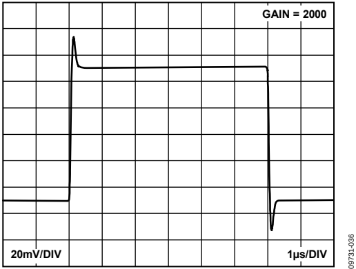
Figure 34. Small Signal Pulse Response, R_L = 10 k \Omega , C_L = 100 pF
