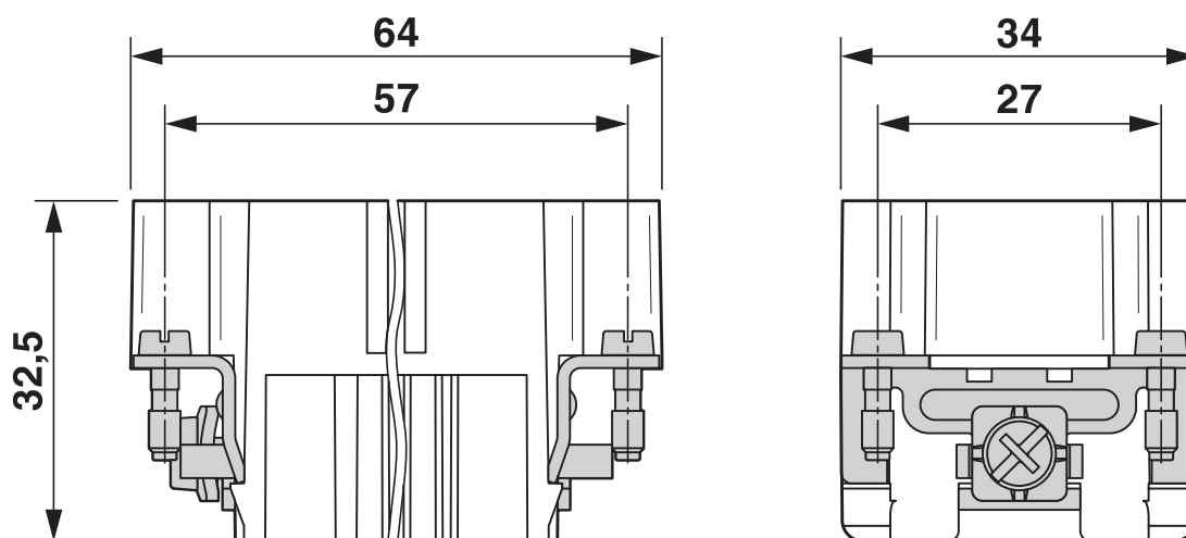
Dimensional drawing
