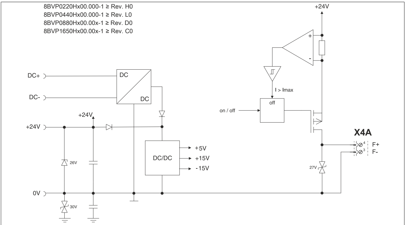
Figure 11: 8BVI fans - Control
