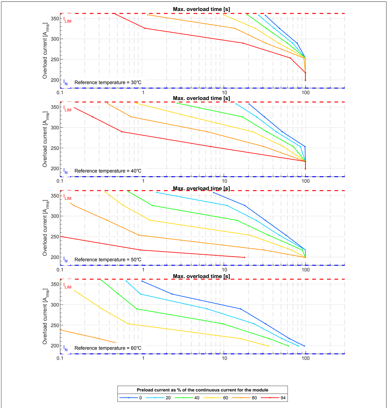
Figure 1: 8BVP1650HC00.004-x - Overload characteristics, overload response - WARNING
