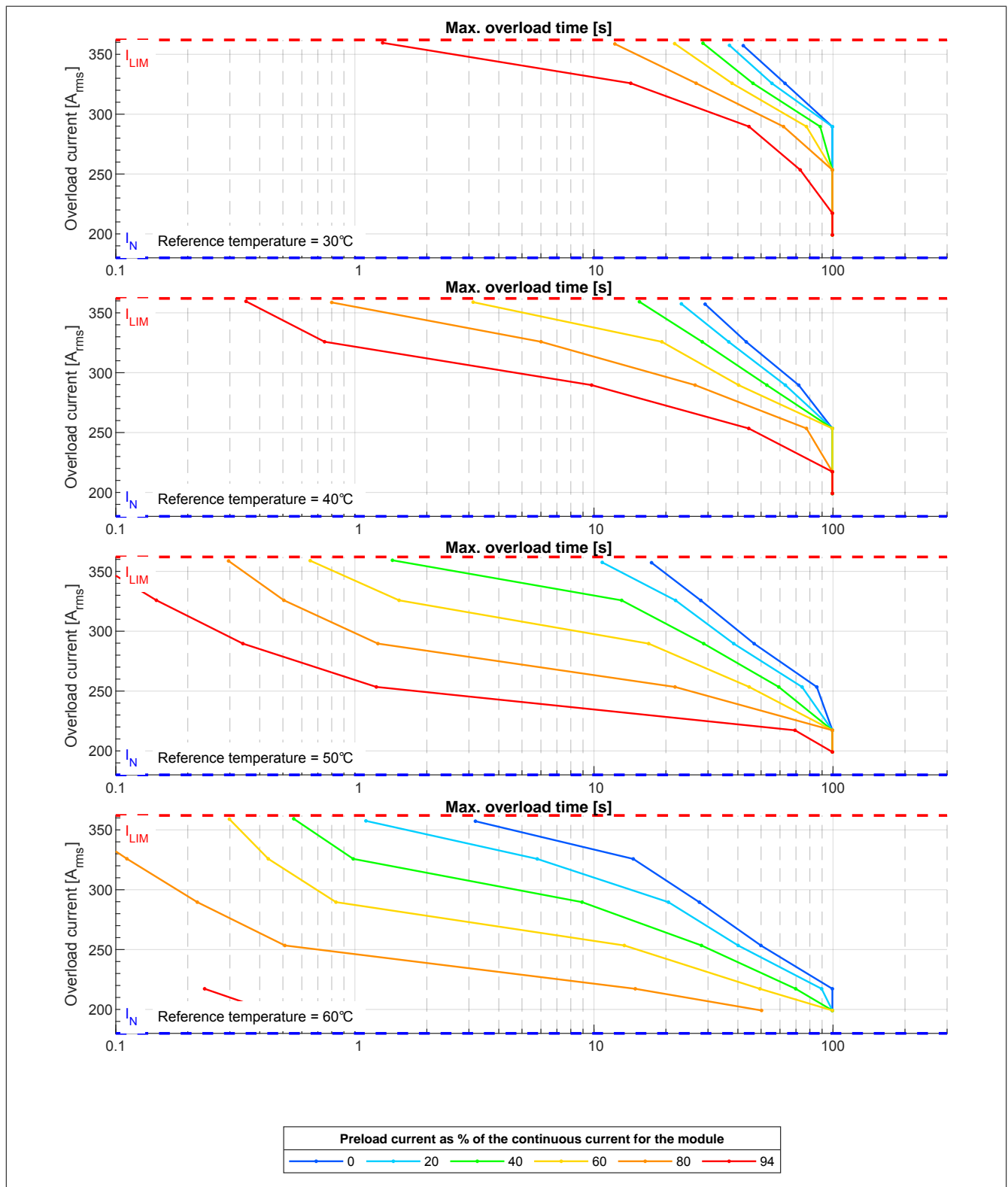
Figure 2: 8BVP1650HC00.004-x - Overload characteristics, overload response - ERROR+STOP
