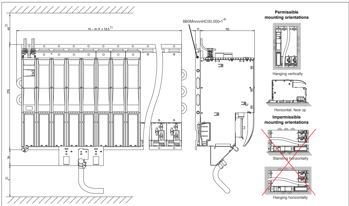
Figure 4: Dimension diagram and installation dimensions
