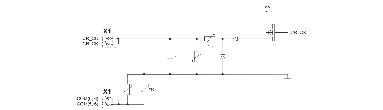
Figure 8: 8B0C enable
