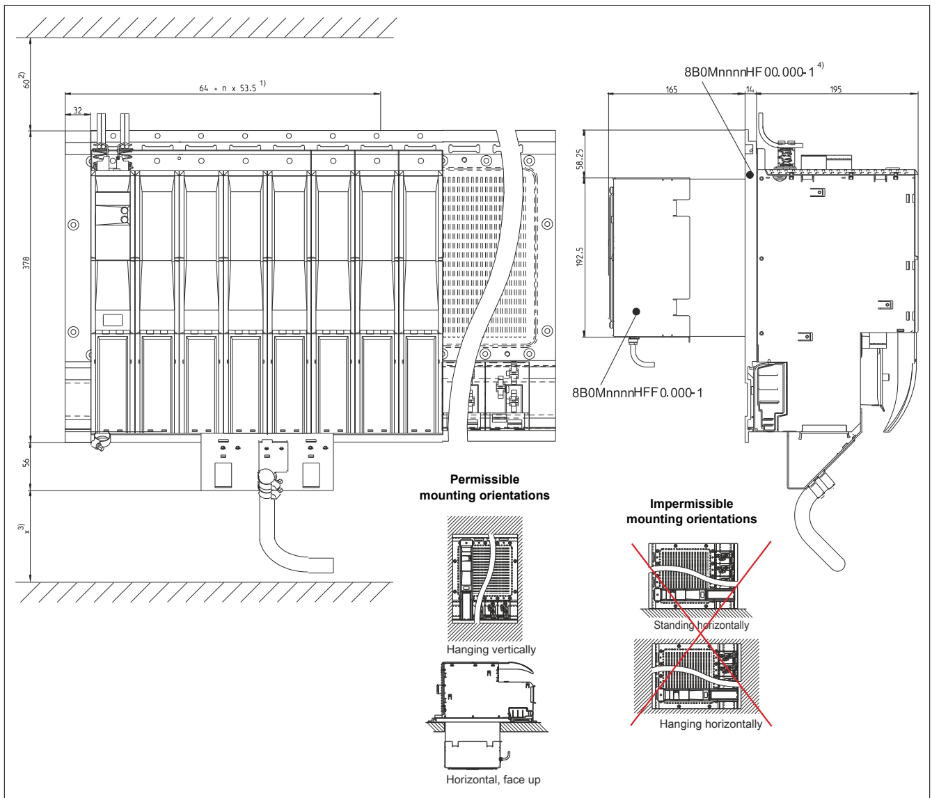
Figure 5: Pass-through mounting - Dimension diagram and installation dimensions
