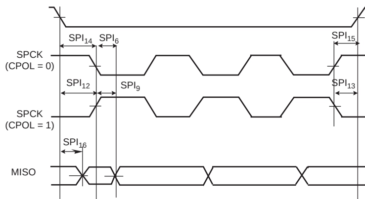
Figure 46-12. SPI Slave Mode - NPCS Timings
