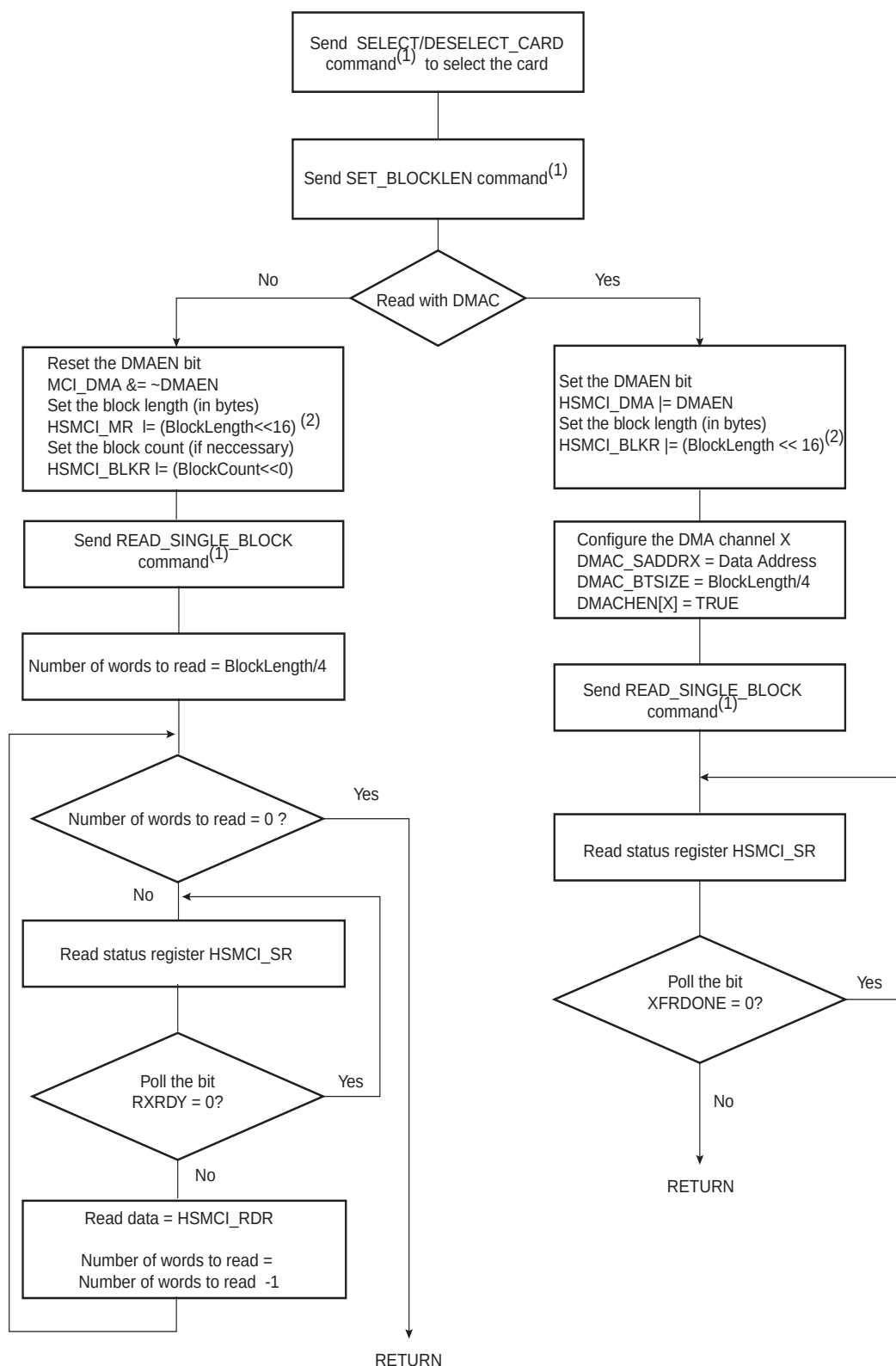
Figure 34-8. Read Functional Flow Diagram
