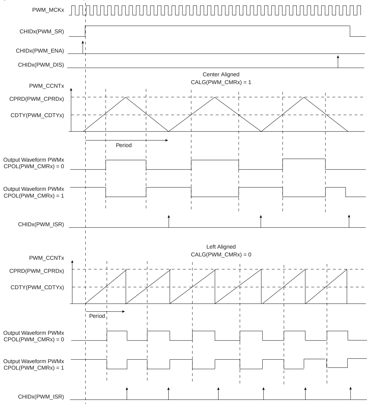
Figure 41-5. Waveform Properties
