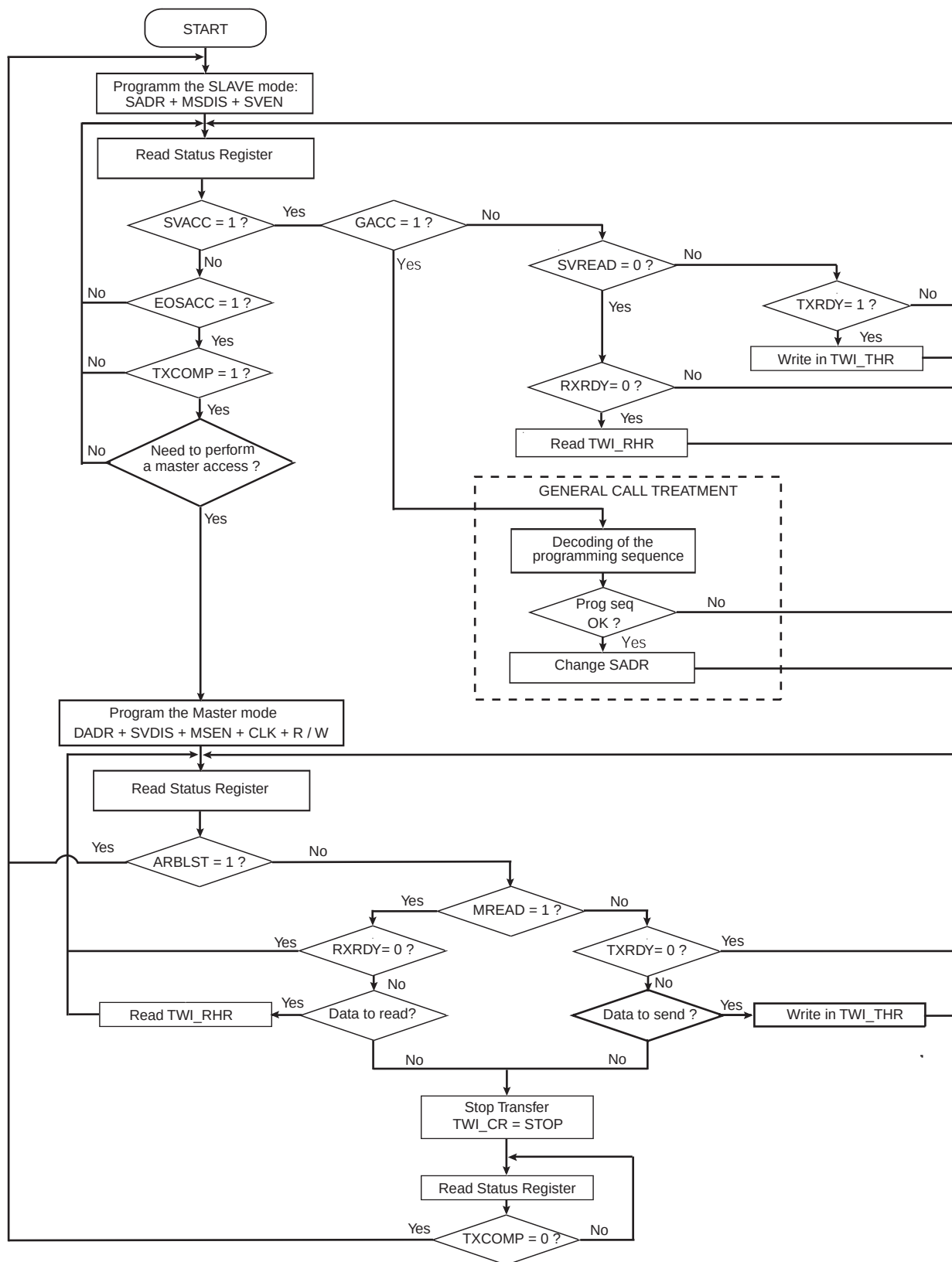
Figure 31-23. Multi-master Flowchart
