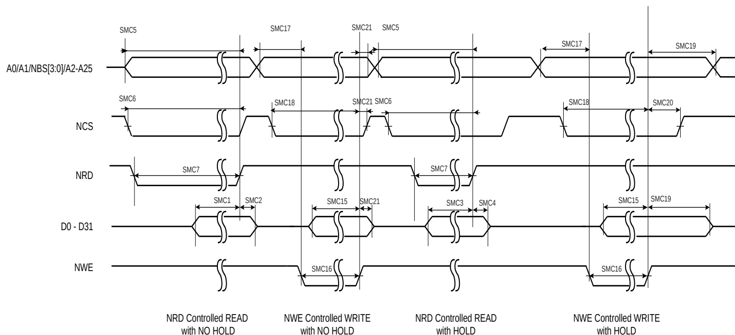
Figure 46-7. SMC Timings - NRD Controlled Read and NWE Controlled Write
