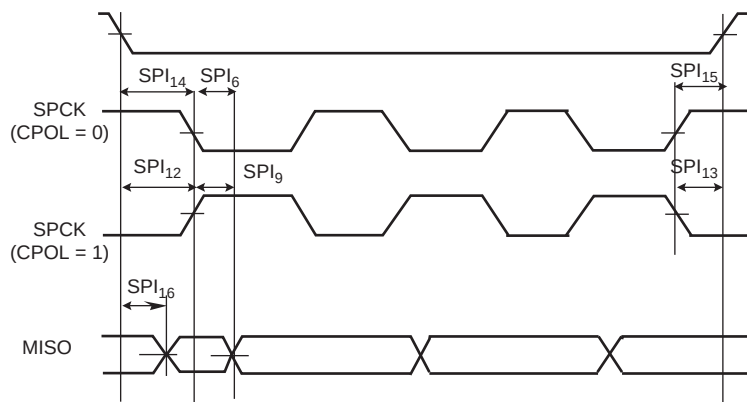
Figure 46-28. SPI Slave Mode - NPCS Timings
