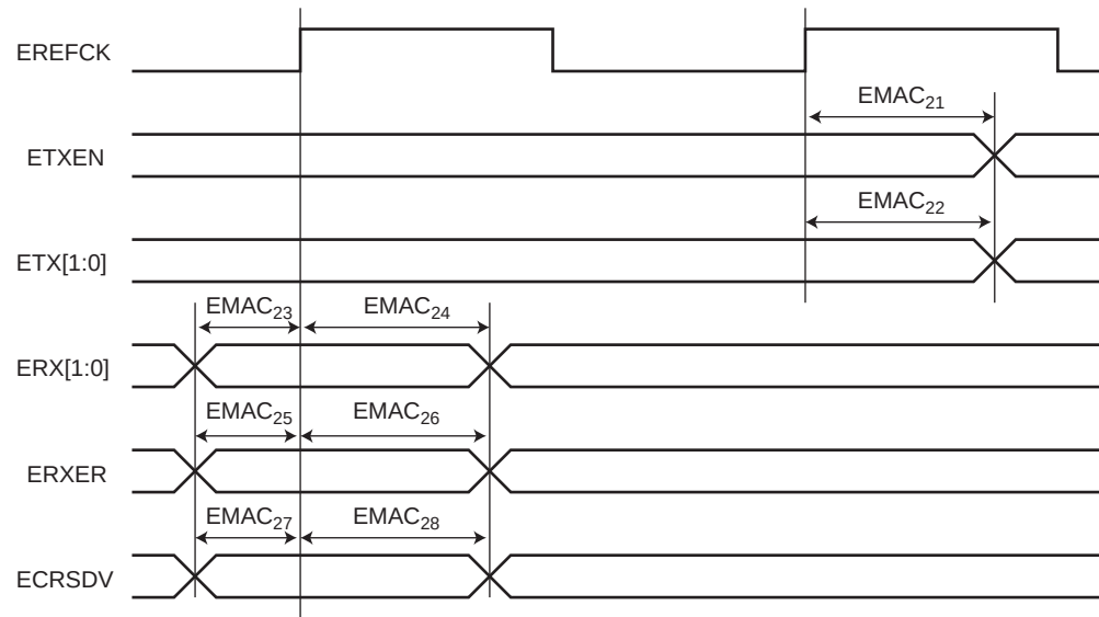
Figure 46-25. EMAC RMII Timings
