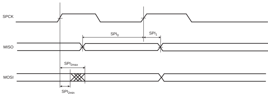
Figure 46-13. Min and Max Access Time for SPI Output Signal
