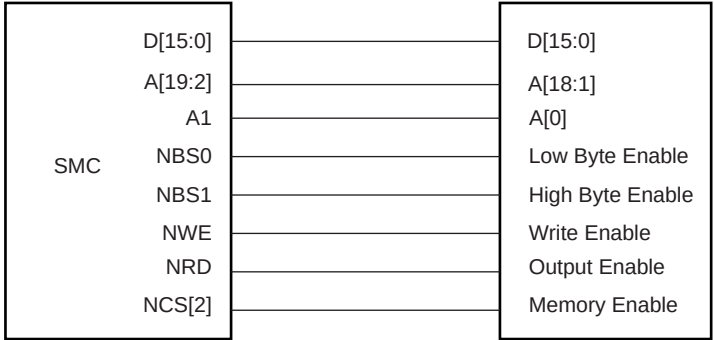
Figure 20-4. Memory Connection for a 16-bit Data Bus
