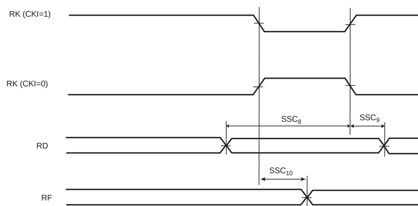
Figure 46-18. SSC Receiver, RK in Input and RF in Output
