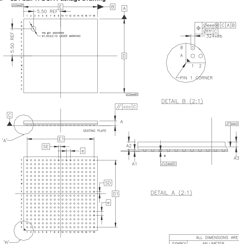
Figure 47-1. 324-ball TFBGA Package Drawing
