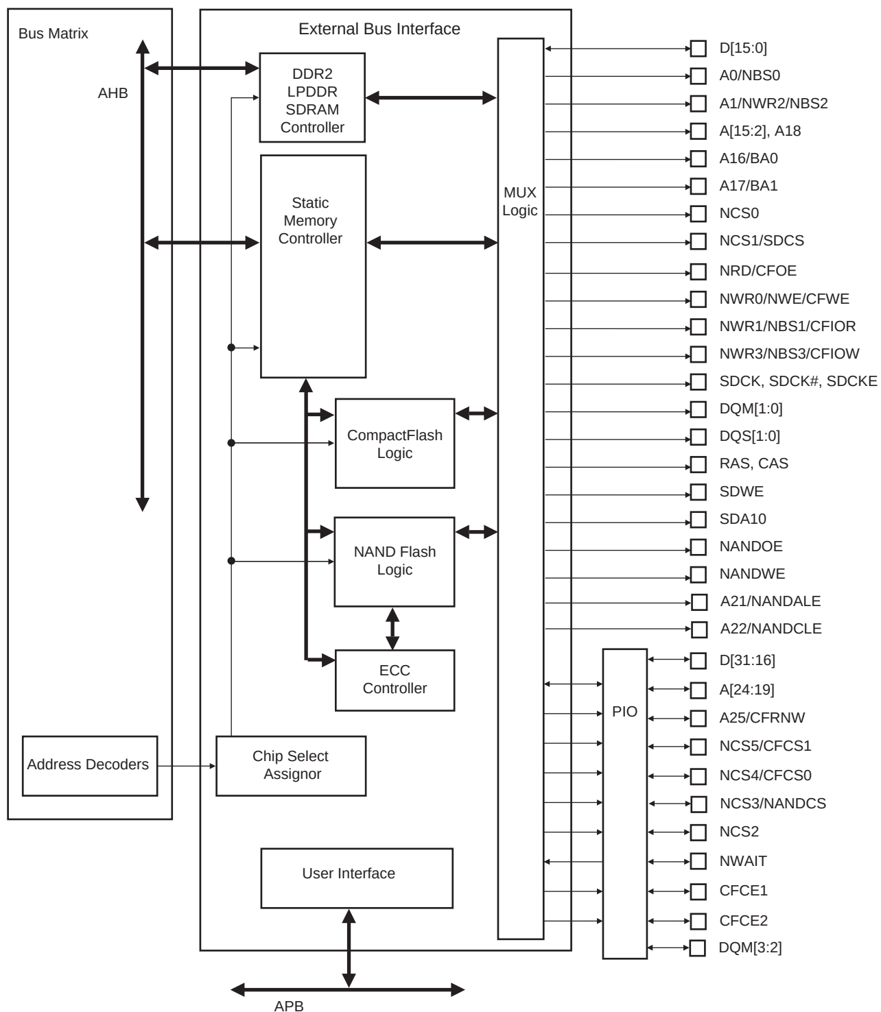
Figure 19-3. Organization of the External Bus Interface
