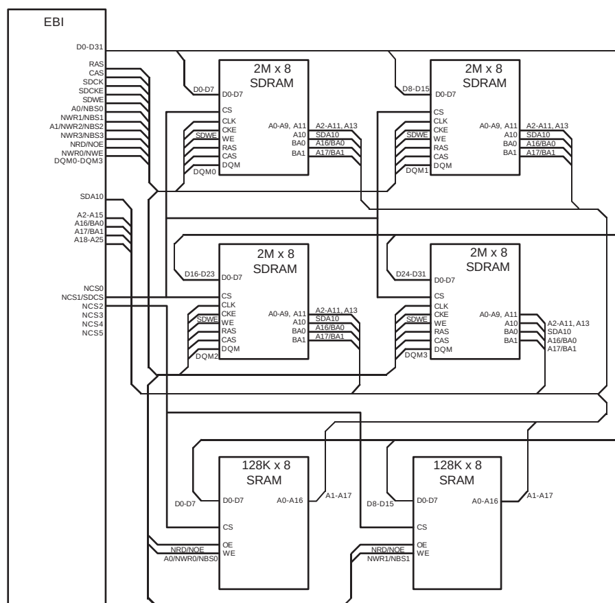
Figure 19-4. EBI Connections to Memory Devices
