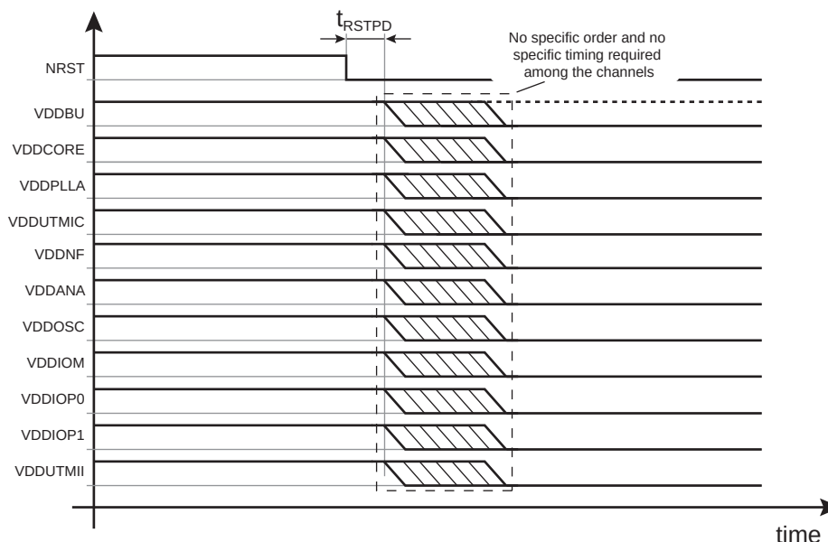
Figure 46-5. Recommended Power-Down Sequence
