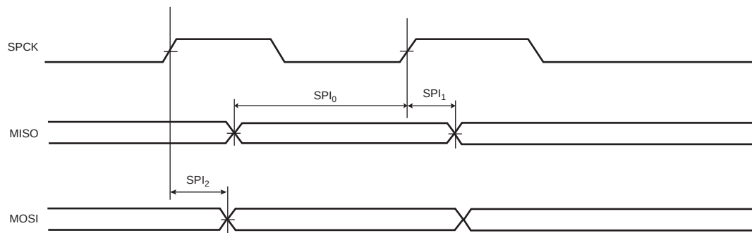
Figure 46-8. SPI Master Mode 1 and 2
