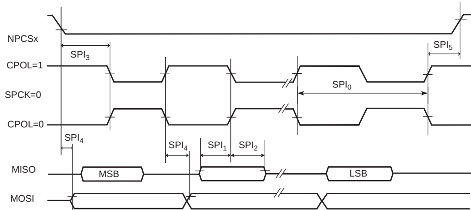
Figure 46-26. UART SPI Master Mode
