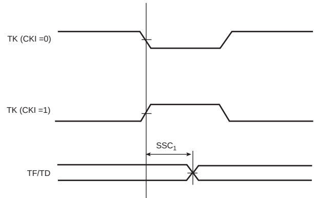
Figure 46-15. SSC Transmitter, TK in Input and TF in Output
