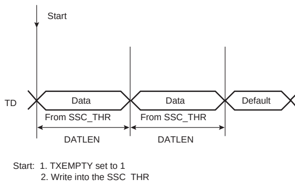
Figure 32-15. Transmit Frame Format in Continuous Mode
