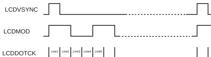
Figure 44-3. Full Frame Timing, MMODE=1, MVAL=1
