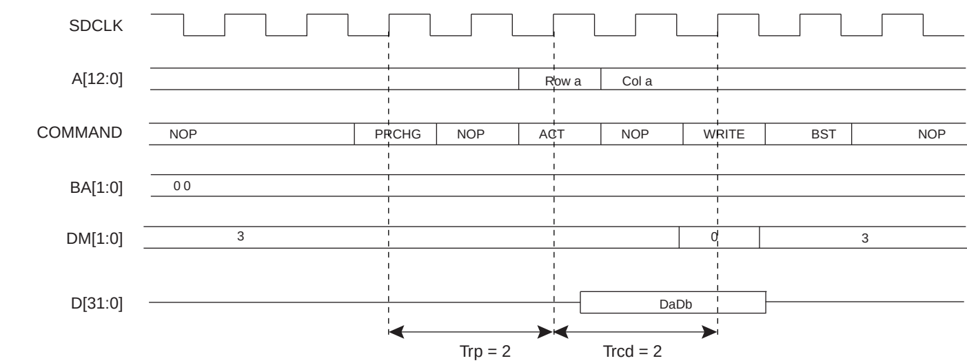
Figure 21-4. Single Write Access, Row Closed, SDR-SDRAM Device
