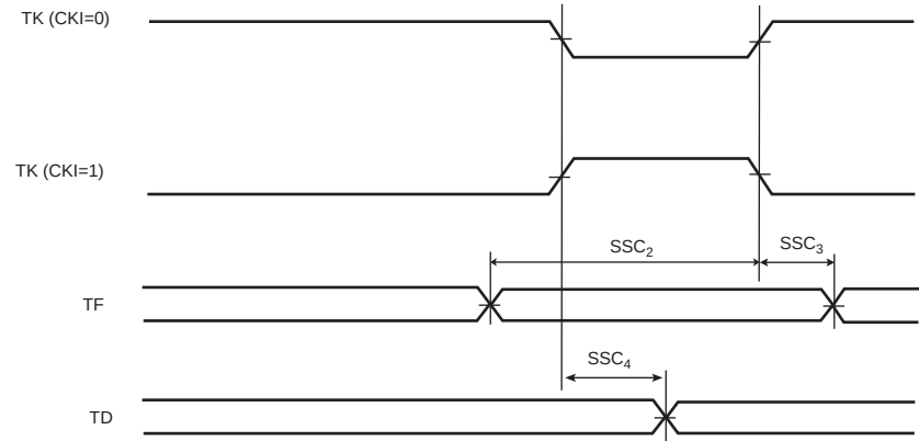
Figure 46-16. SSC Transmitter, TK in Output and TF in Input
