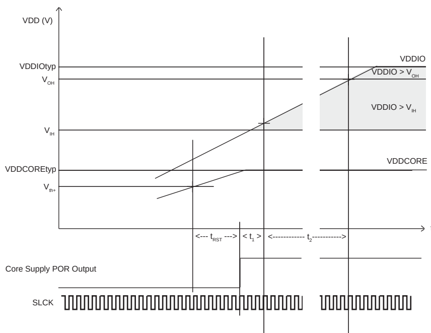
Figure 46-4. VDDCORE and VDDIO Constraints at Startup
