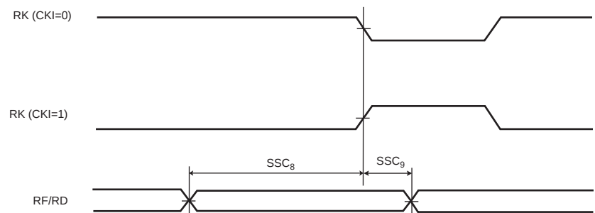
Figure 46-17. SSC Receiver RK and RF in Input
