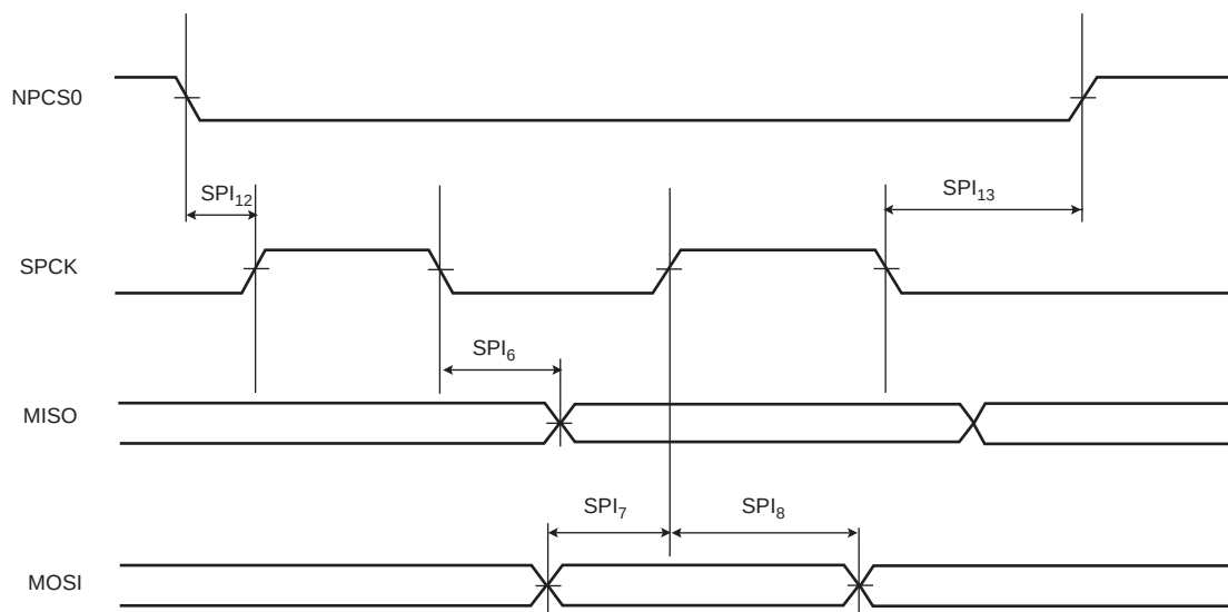
Figure 46-27. UART SPI Slave Mode
