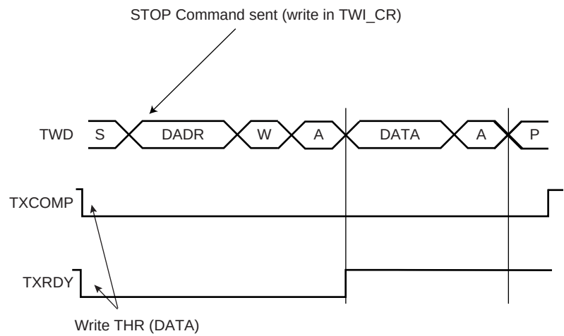
Figure 31-6. Master Write with One Data Byte
