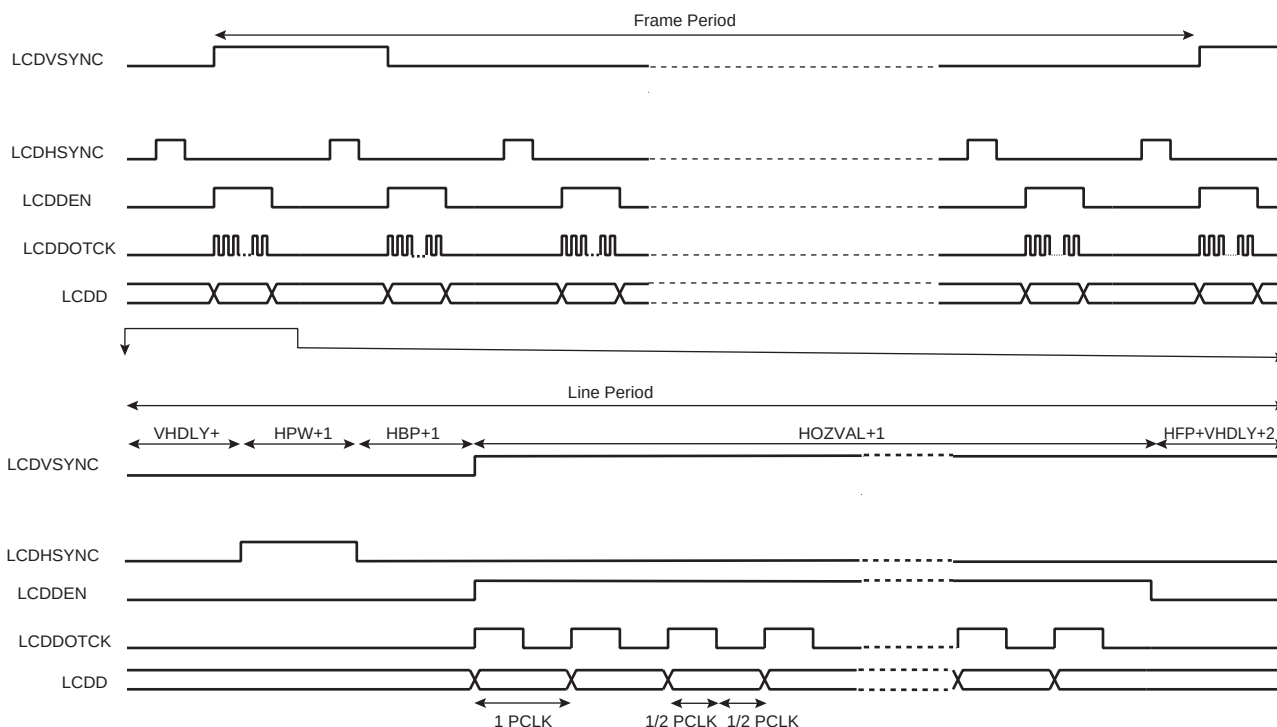
Figure 44-5. STN Panel Timing, CLKMOD 0
