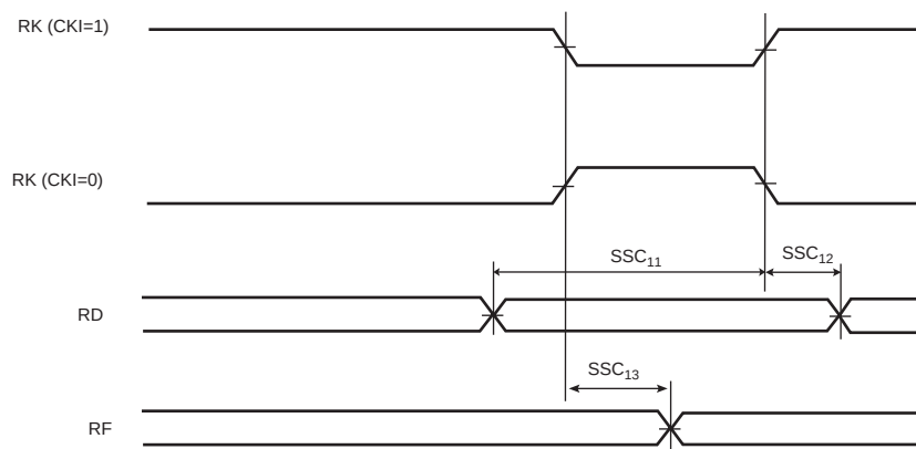
Figure 46-19. SSC Receiver, RK and RF in Output
