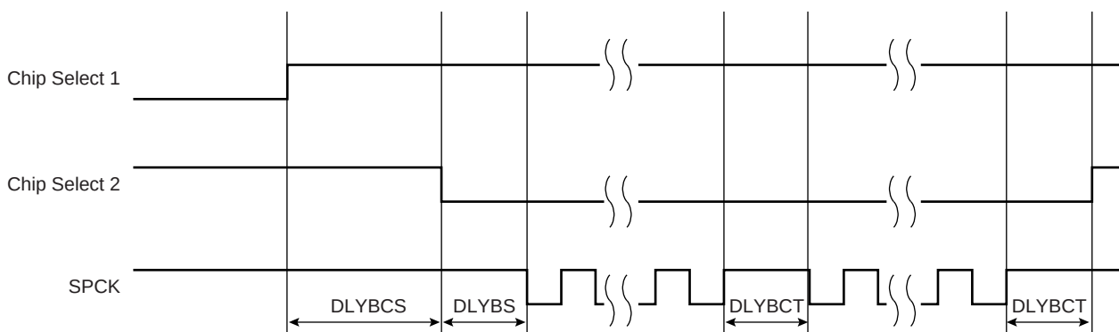
Figure 26-10. Programmable Delays
