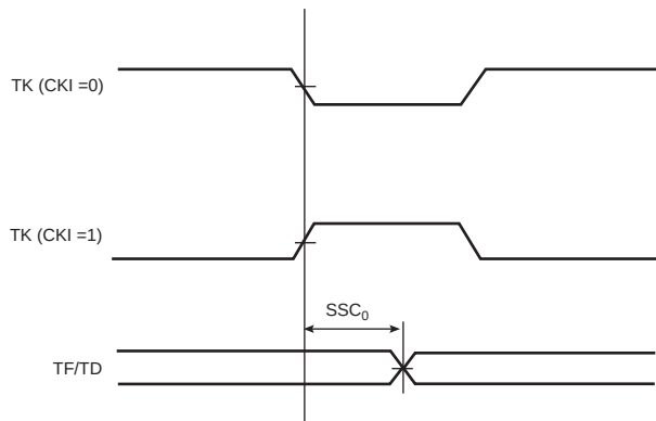
Figure 46-14. SSC Transmitter, TK and TF in Output
