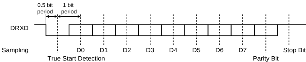
Figure 28-5. Character Reception Example: 8-bit, parity enabled 1 stop
