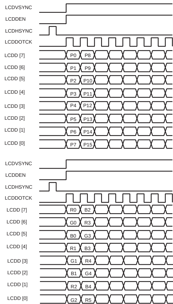
Figure 44-10. Single Scan Monochrome and Color 8-bit Panel Timing (First Line Expanded View)
