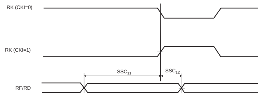
Figure 46-20. SSC Receiver, RK in Output and RF in Input
