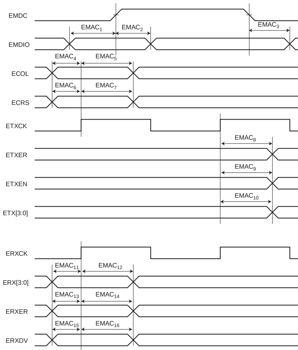
Figure 46-24. EMAC MII Mode
