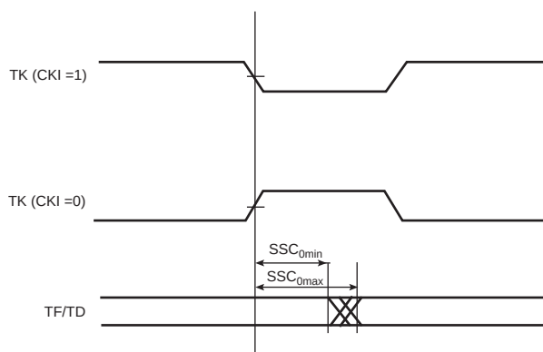
Figure 46-21. Min and Max Access Time of Output Signals
