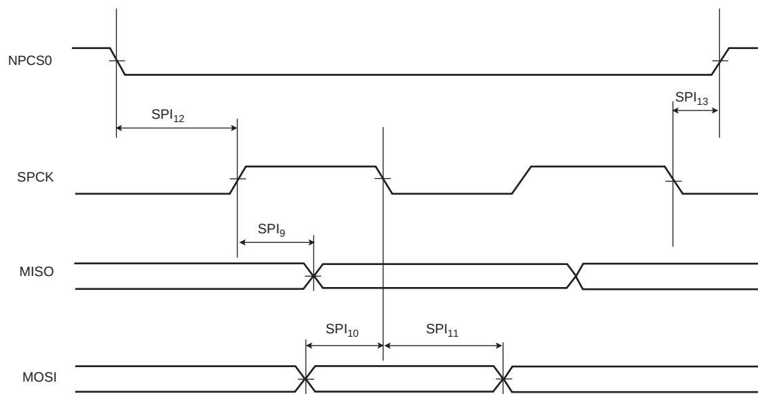
Figure 46-11. SPI Slave Mode 1 and 2
