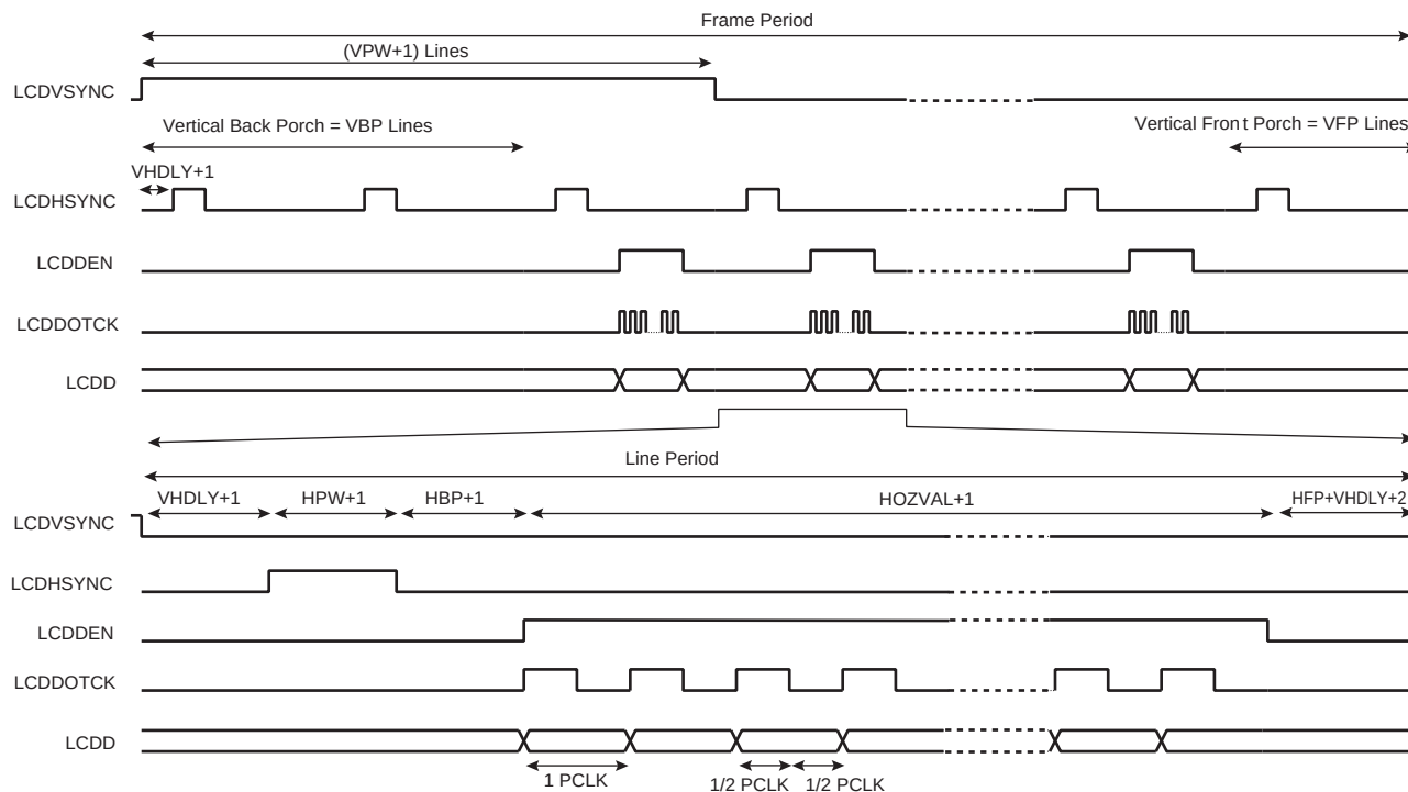
Figure 44-6. TFT Panel Timing, CLKMOD = 0, VPW = 2, VBP = 2, VFP = 1
