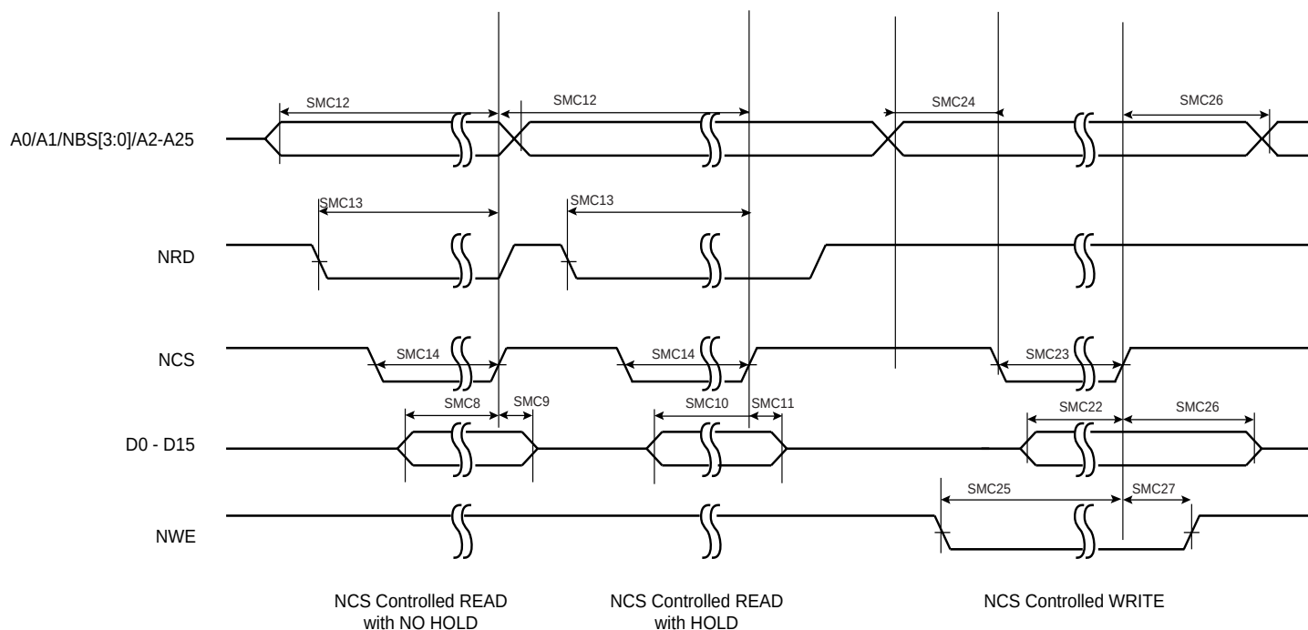
Figure 46-6. SMC Timings - NCS Controlled Read and Write
