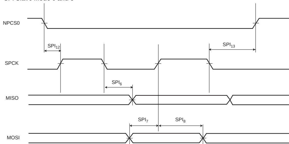
Figure 46-10. SPI Slave Mode 0 and 3
