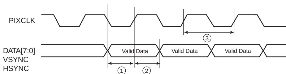
Figure 46-22. ISI Timing Diagram
