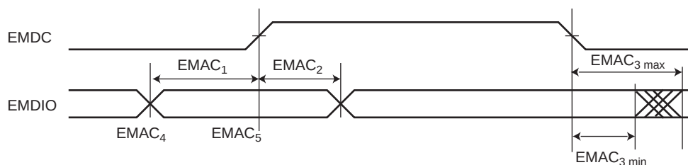
Figure 46-23. Min and Max Access Time of EMAC Output Signals
