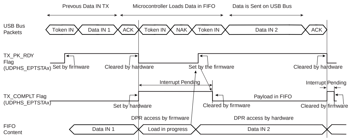
Figure 37-9. Data IN Transfer for Endpoint with Two Banks
