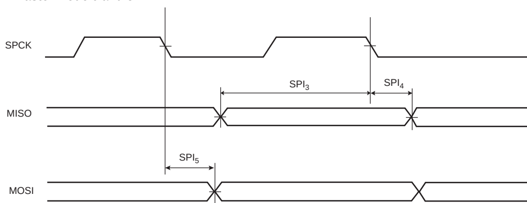
Figure 46-9. SPI Master Mode 0 and 3
