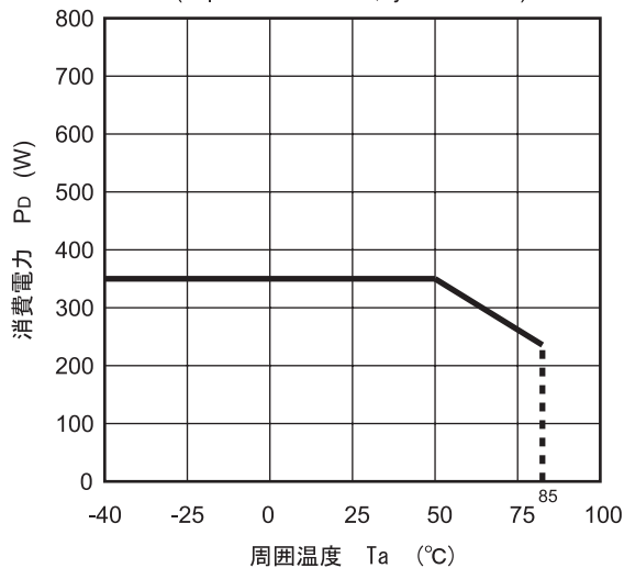
消費電力—周囲温度特性例 ( T_{opr} = -40 \sim +85^\circ\text{C} , T_j = \sim +150^\circ\text{C} )
