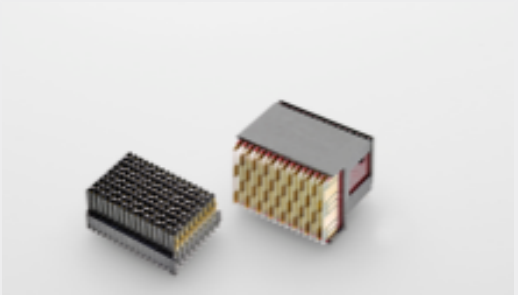
TE Part #2302785-1 RA PLUG ASSY,7ROW,CENTER,VPX, MG RT3
