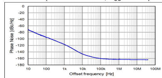
Phase Noise (fo = 156.25 MHz, V_{CC} = 3.3 V)
