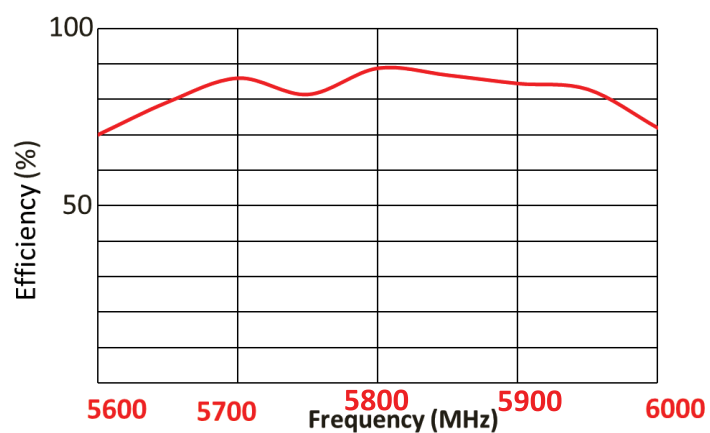
Efficiency
