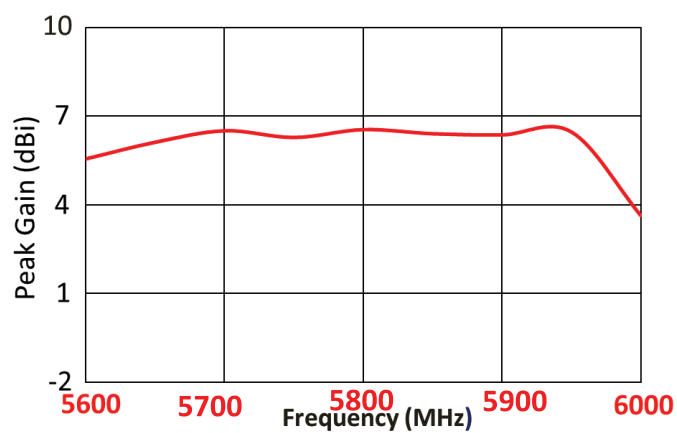
Peak Gain
