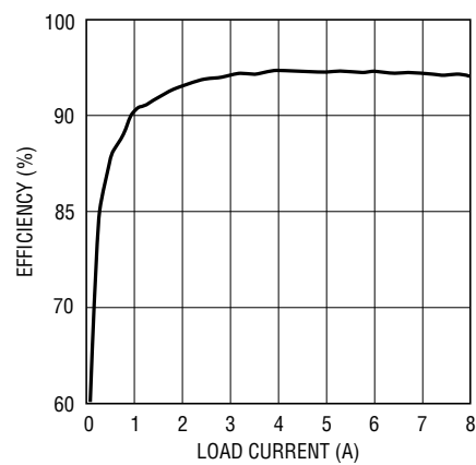
12V OUT Efficiency vs Load Currnt
