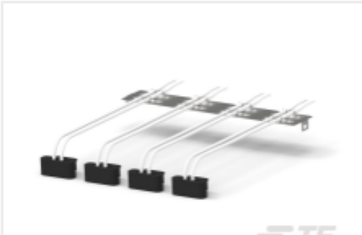
TE Part #2325080-5 LIGHTPIPE ASSEMBLY, OSFP
