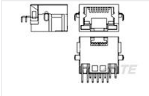
TE Part #2041126-1 MODULAR JACK, RJ45, SMT TYPE,AU: 6u"
