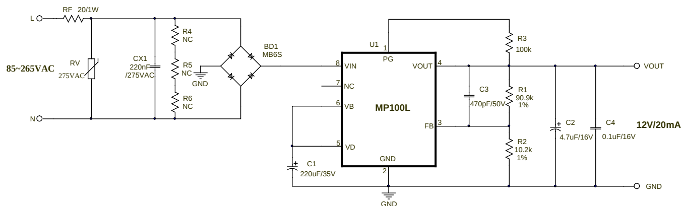
Figure 4: Typical Application
