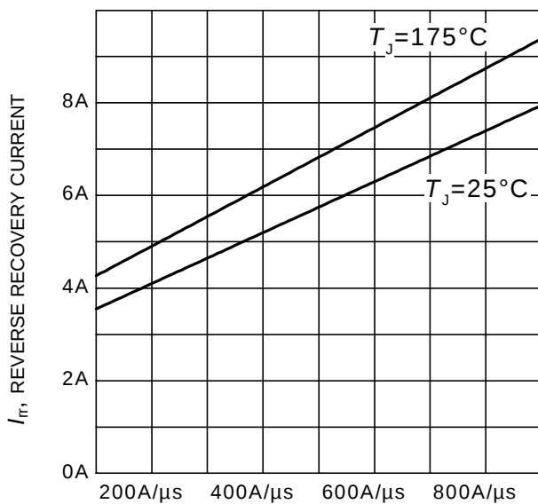
Figure 25. Typical reverse recovery current as a function of diode current slope ( V_R = 400V , I_F = 6A , Dynamic test circuit in Figure E)
