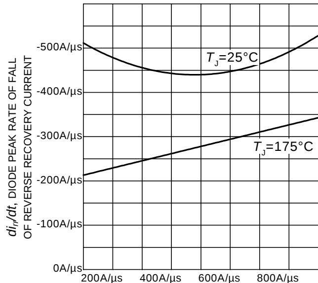
Figure 26. Typical diode peak rate of fall of reverse recovery current as a function of diode current slope ( V_R = 400V , I_F = 6A , Dynamic test circuit in Figure E)
