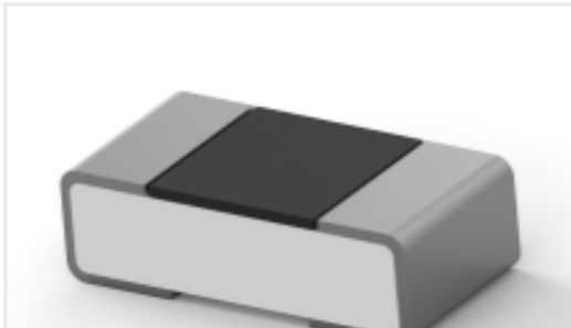
TE Part #5-2176364-0 RQ 0402 15K 0.1% 10PPM 5K RL
