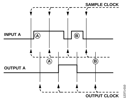
Figure 10. Low Speed Channel Timing
