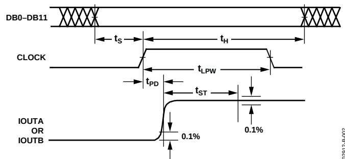
Figure 2. Timing Diagram
