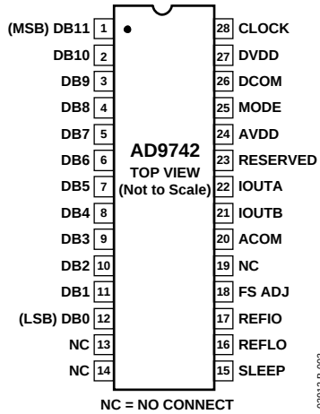
Figure 3. 28-Lead SOIC and TSSOP Pin Configuration
