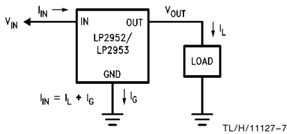
FIGURE 1. Current/Voltage Diagram
