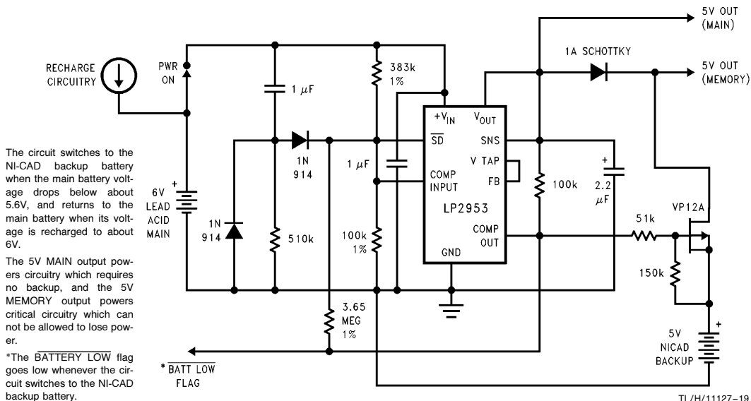
5V Battery Powered Supply with Backup and Low Battery Flag
