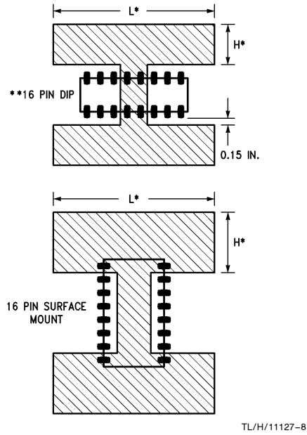
FIGURE 2. Copper Heatsink Patterns
