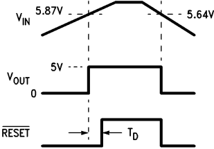
Timing Diagram
