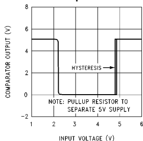
Dropout Detection Comparator Threshold Voltages
