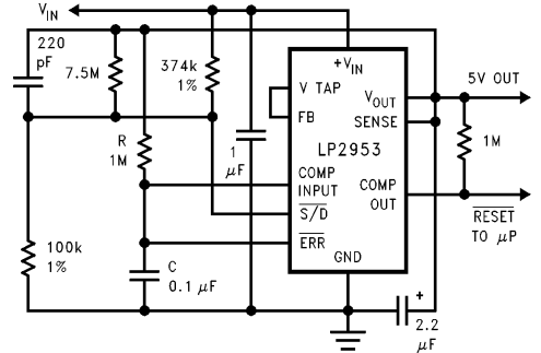
5V Regulator with Timed Power-On Reset, Snap-On/Snap-Off Feature and Hysteresis
