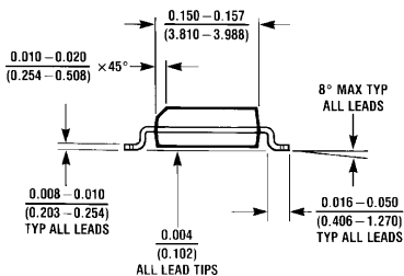
16-Pin Surface Mount Order Number LP2952IM, LP2952AIM, LP2952IM-3.3, LP2952AIM-3.3, LP2953IM, LP2953AIM, LP2953IM-3.3 or LP2953AIM-3.3 NS Package Number M16A
