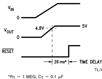
Timing Diagram for Timed Power-On Reset
