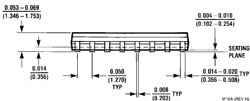
16-Pin Surface Mount Order Number LP2952IM, LP2952AIM, LP2952IM-3.3, LP2952AIM-3.3, LP2953IM, LP2953AIM, LP2953IM-3.3 or LP2953AIM-3.3 NS Package Number M16A
