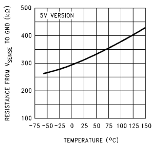
Divider Resistance
