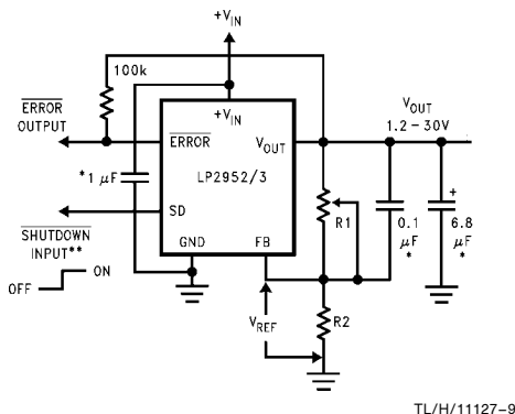
FIGURE 4. Adjustable Regulator
