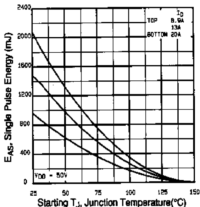
Fig 12c. Maximum Avalanche Energy Vs. Drain Current
