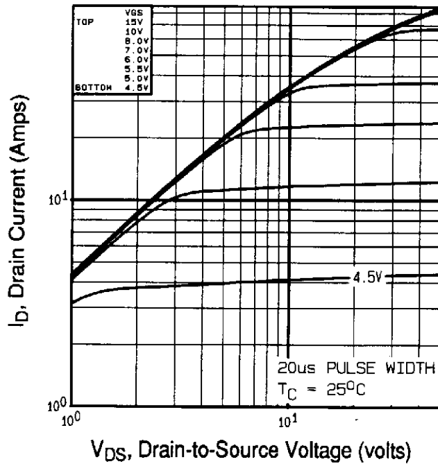
Fig 1. Typical Output Characteristics, T_C=25^\circ\text{C}
