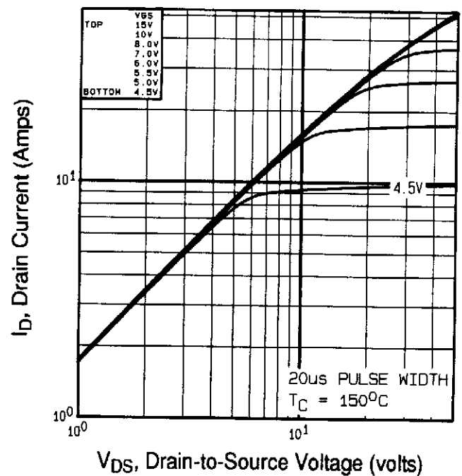
Fig 2. Typical Output Characteristics, T_C=150^\circ\text{C}
