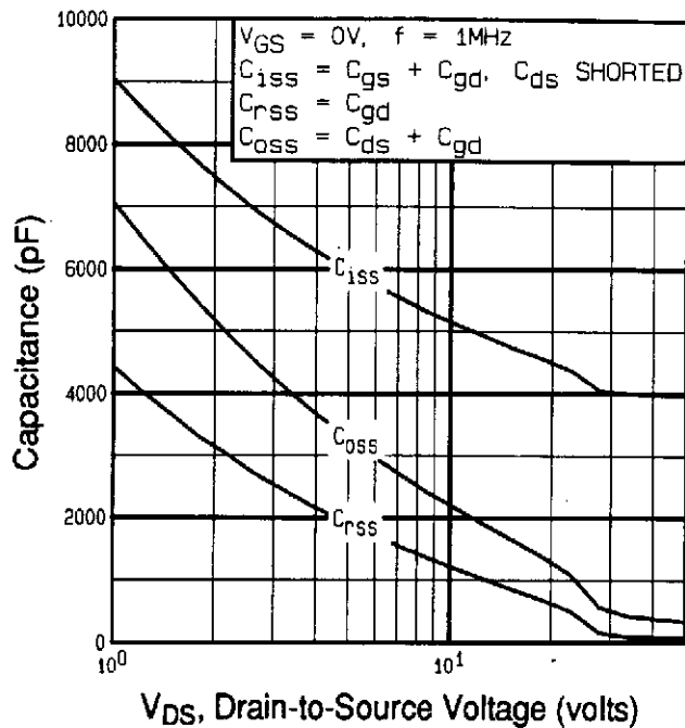
Fig 5. Typical Capacitance Vs. Drain-to-Source Voltage
