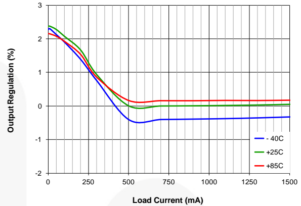
Figure 12. Output Regulation vs. Load Current and Temperature (Normalized to 3.6 V_{IN} , 500 mA Load, T_A=25^\circ\text{C} )
