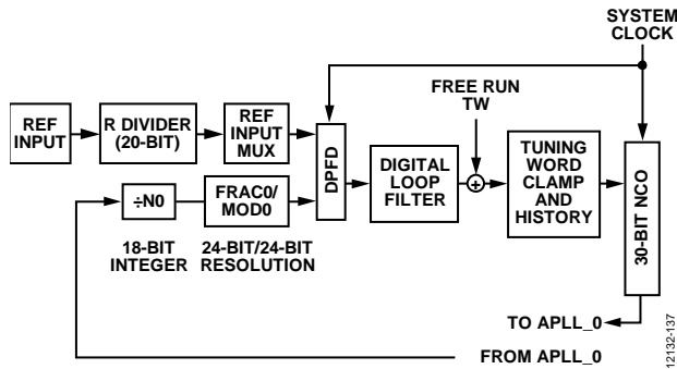
Figure 27. DPLL_0 Core
