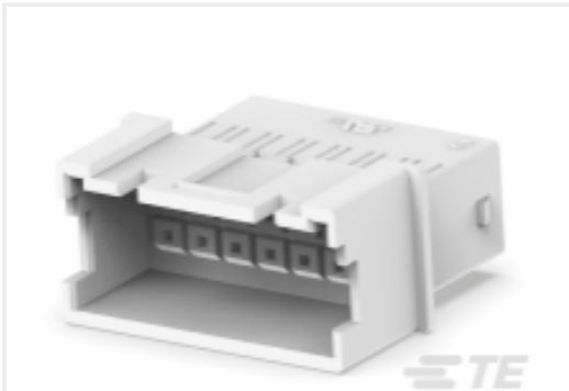
TE Part # 1-2324201-4 HSG,REC,FREE-HANGING,GWT, DUALROW,EP2.5
