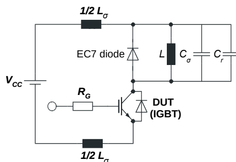
Figure C. Dynamic test circuit
