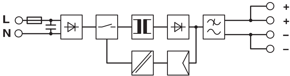
Block diagram
