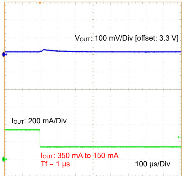
Figure 46. Load Transient 350 mA to 150 mA (3.3 V Output, Tf = 1\text{ }\mu\text{s} )
