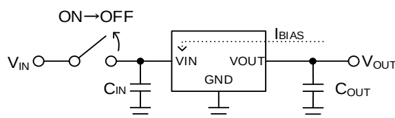
Figure 60. Open VIN
