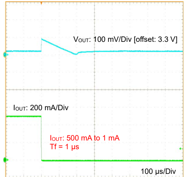
Figure 44. Load Transient 500 mA to 1 mA (3.3 V Output, Tf = 1\text{ }\mu\text{s} )
