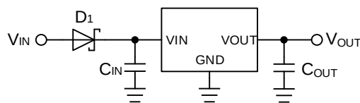
Figure 62. Protection against Reverse Polarity 1
