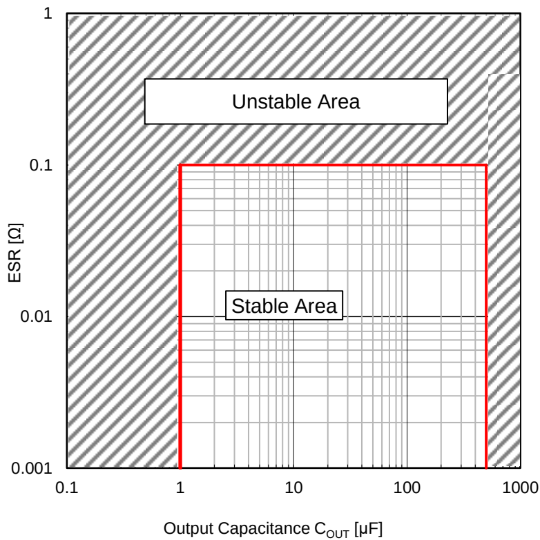
Figure 55. Output Capacitance C_{OUT} , ESR Available Area ( V_{IN} = 4.5\text{ V} to 42\text{ V} , V_{OUT} = 1\text{ V} (Note 1) , -40\text{ }^{\circ}\text{C} \leq T_j \leq +150\text{ }^{\circ}\text{C} , I_{OUT} = 0\text{ mA} to 500\text{ mA} ) (Note 1) The most strict condition from the stability theory for the control loop of regulator.
