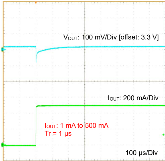
Figure 43. Load Transient 1 mA to 500 mA (3.3 V Output, Tr = 1\text{ }\mu\text{s} )
