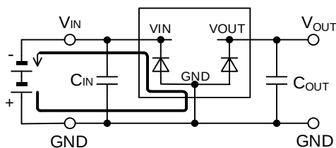
Figure 61. Current Path in Reverse Input Connection
