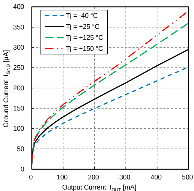
Figure 33. Ground Current vs Output Current (3.3 V Output)
