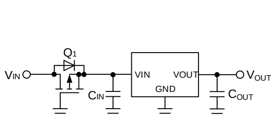
Figure 63. Protection against Reverse Polarity 2
