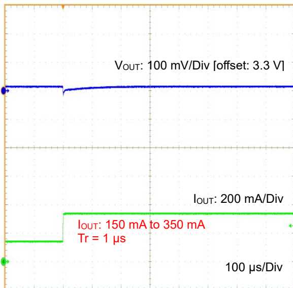
Figure 45. Load Transient 150 mA to 350 mA (3.3 V Output, Tr = 1\text{ }\mu\text{s} )
