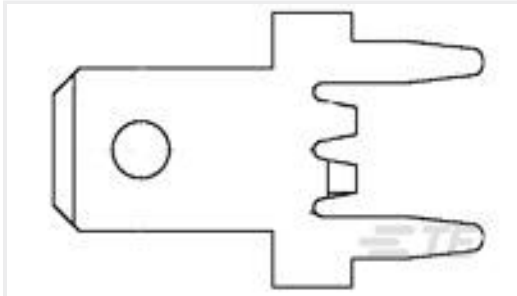
TE Part #63860-1 187 FASTON TAB TPBR
