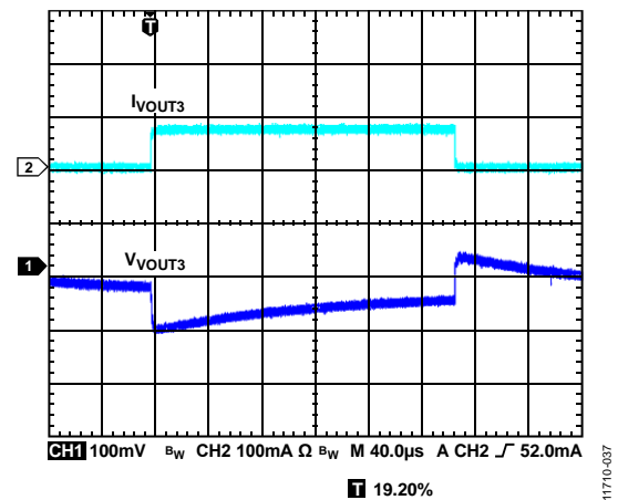
Figure 37. LDO Response to Load Transient, I_{OUT3} from 1 mA to 80 mA, V_{VOUT3} = 2.8\text{ V}
