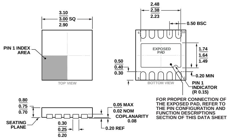
Figure 75. 10-Lead Lead Frame Chip Scale Package [LFCSP_WD] 3 mm × 3 mm Body, Very Very Thin, Dual Lead (CP-10-9)
