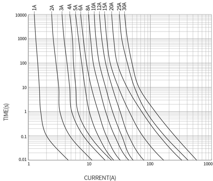
HC10PV AVERAGE I-T CHARACTERISTICS CURVE (FOR REFERENCE ONLY)
