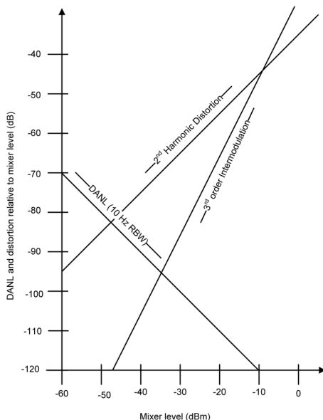
Nominal Dynamic Range at 1 GHz
