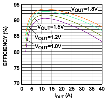
Device Efficiency vs. Output Current L=FP1007R3-R22-R
