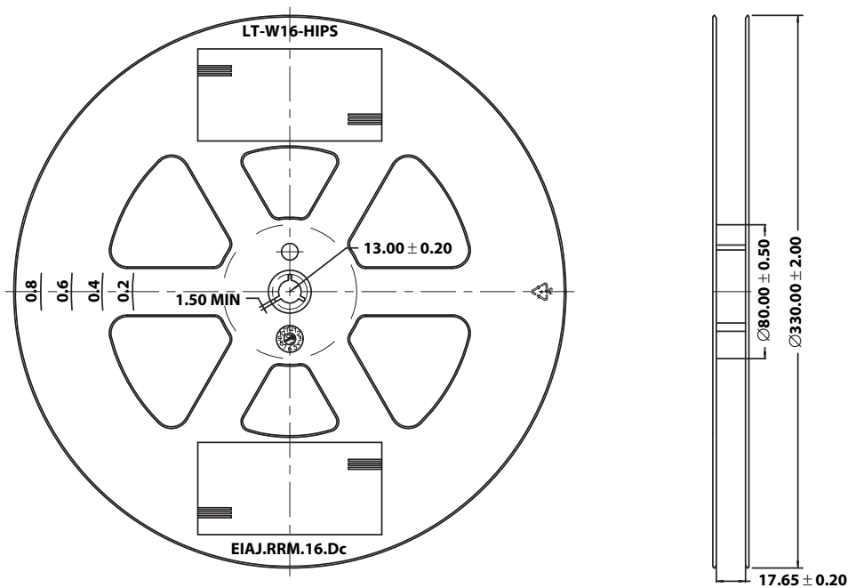
Figure 19. Reel Dimension
