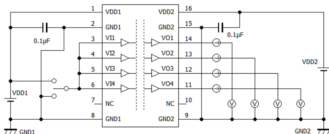
Fig.12-2-1. DCL540C01/DCL540D01 VOH/VOL Test Circuit
