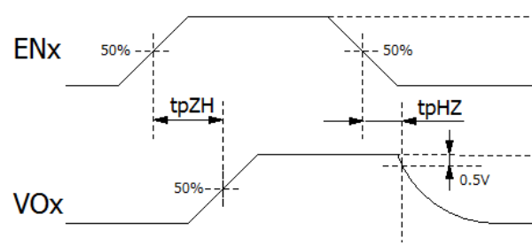
Fig.12-5. DCL540L01/ DCL540H01 Enable Propagation Delay Time Test Circuit and Waveforms
