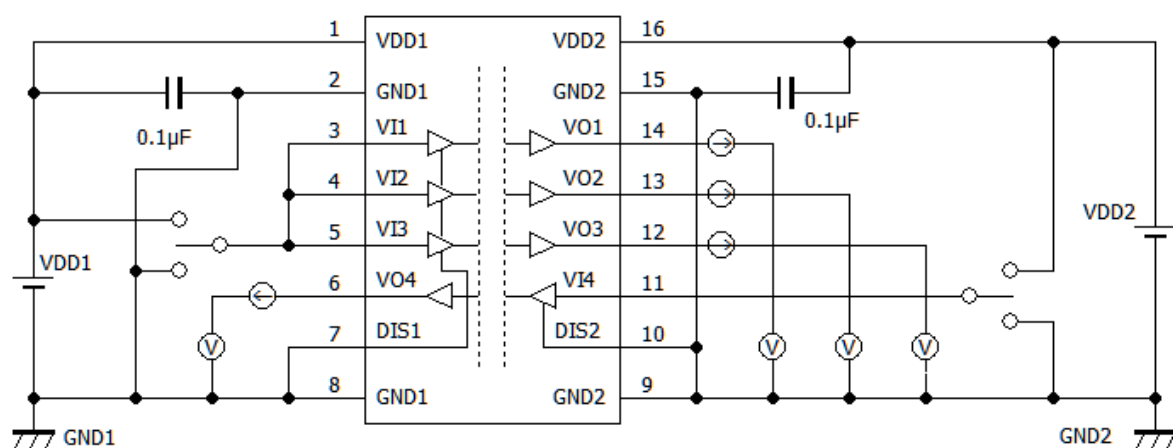
Fig.12-2-3. DCL541A01/DCL541B01 VOH/VOL Test Circuit
