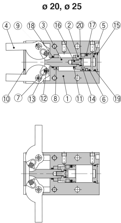
Component Parts
